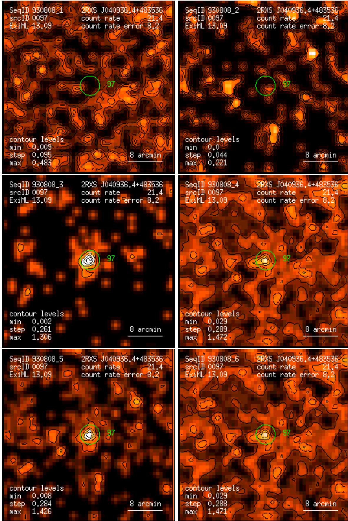
Figure 97: RASS 930808: detection 0097: band rate images, Gaussian filter: (1) PSPC channels 11 – 41, (2) 52 – 90, (3) 91 – 201, (4) 11 – 235, (5) 52 – 201, (6) 11 – 201. Broad band rates in counts/ks. Band rate contour levels in counts/ks/arcmin 2 .
