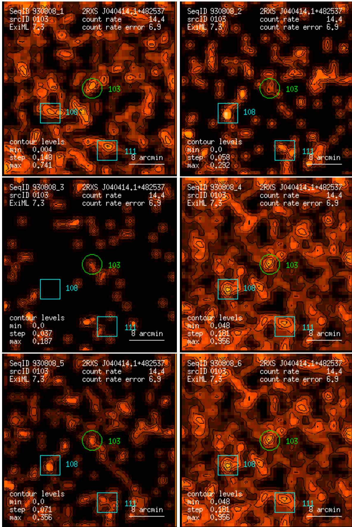
Figure 103: RASS 930808: detection 0103: band rate images, Gaussian filter: (1) PSPC channels 11 – 41, (2) 52 – 90, (3) 91 – 201, (4) 11 – 235, (5) 52 – 201, (6) 11 – 201. Broad band rates in counts/ks. Band rate contour levels in counts/ks/arcmin 2 .
