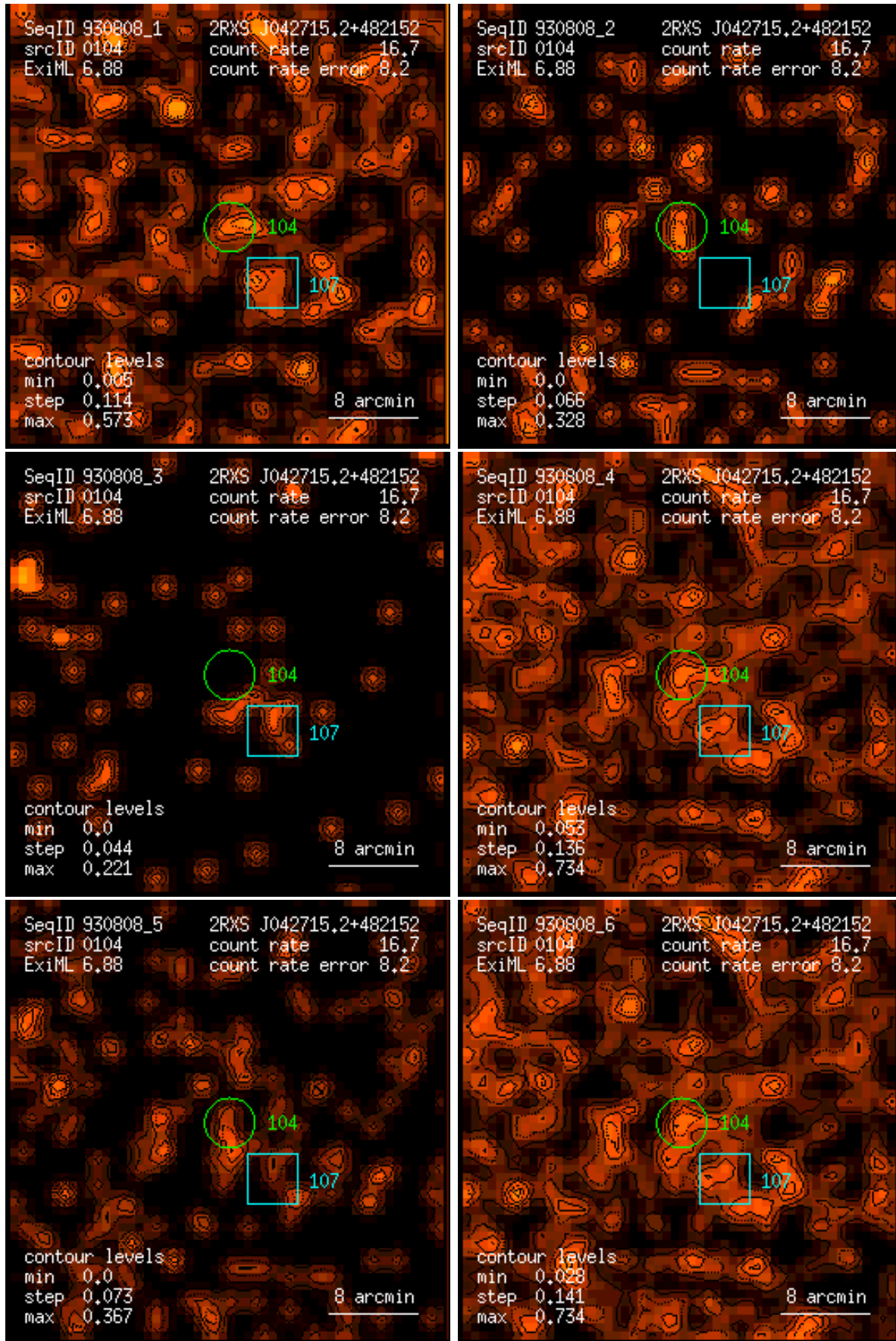
Figure 104: RASS 930808: detection 0104: band rate images, Gaussian filter: (1) PSPC channels 11 – 41, (2) 52 – 90, (3) 91 – 201, (4) 11 – 235, (5) 52 – 201, (6) 11 – 201. Broad band rates in counts/ks. Band rate contour levels in counts/ks/arcmin 2 .
