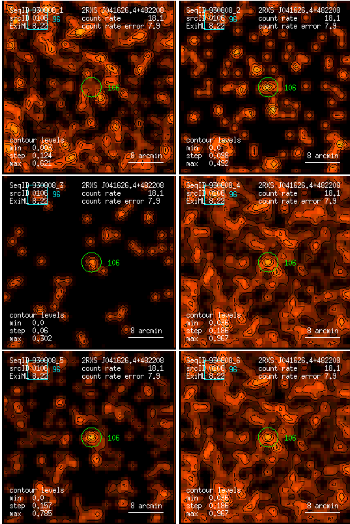
Figure 106: RASS 930808: detection 0106: band rate images, Gaussian filter: (1) PSPC channels 11 – 41, (2) 52 – 90, (3) 91 – 201, (4) 11 – 235, (5) 52 – 201, (6) 11 – 201. Broad band rates in counts/ks. Band rate contour levels in counts/ks/arcmin 2 .
