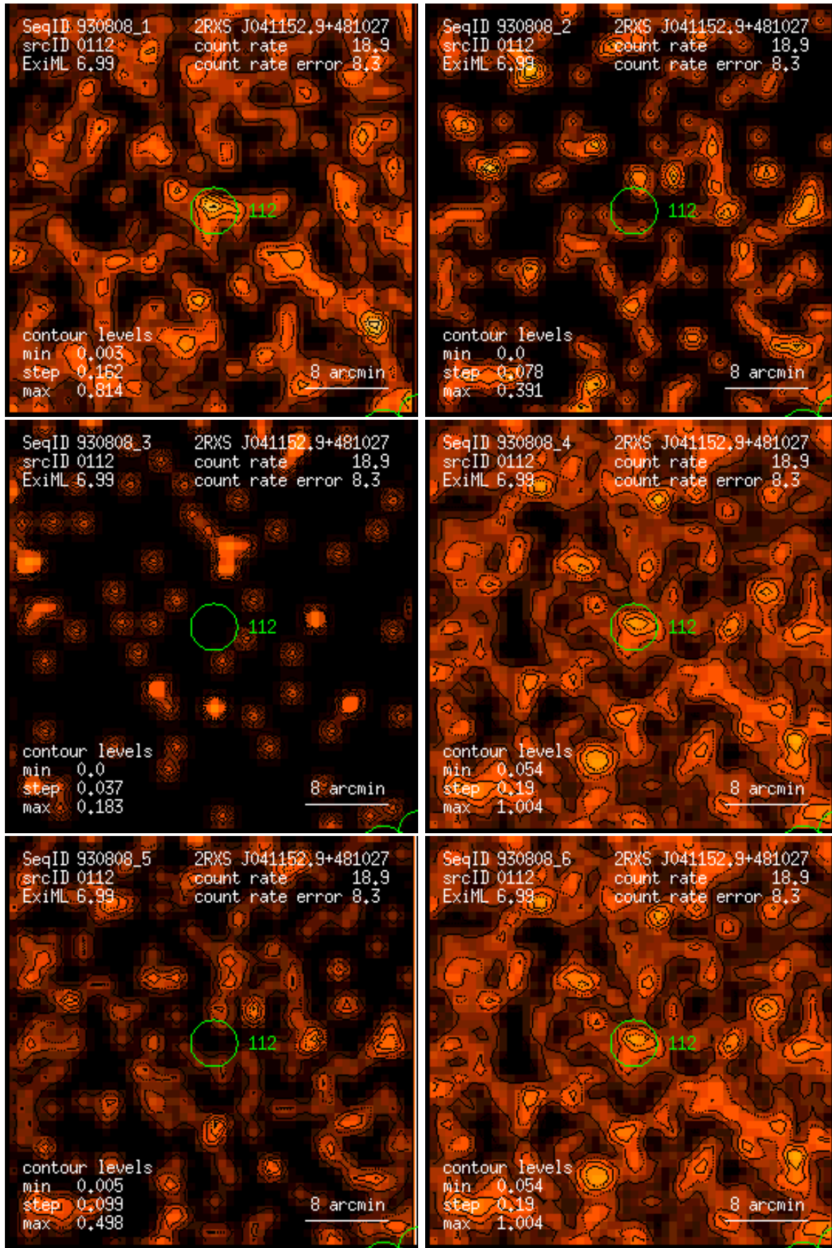
Figure 112: RASS 930808: detection 0112: band rate images, Gaussian filter: (1) PSPC channels 11 – 41, (2) 52 – 90, (3) 91 – 201, (4) 11 – 235, (5) 52 – 201, (6) 11 – 201. Broad band rates in counts/ks. Band rate contour levels in counts/ks/arcmin 2 .
