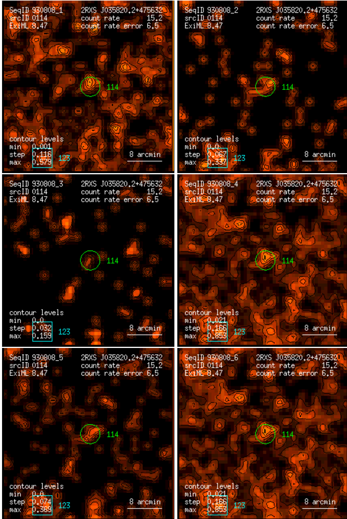
Figure 114: RASS 930808: detection 0114: band rate images, Gaussian filter: (1) PSPC channels 11 – 41, (2) 52 – 90, (3) 91 – 201, (4) 11 – 235, (5) 52 – 201, (6) 11 – 201. Broad band rates in counts/ks. Band rate contour levels in counts/ks/arcmin 2 .
