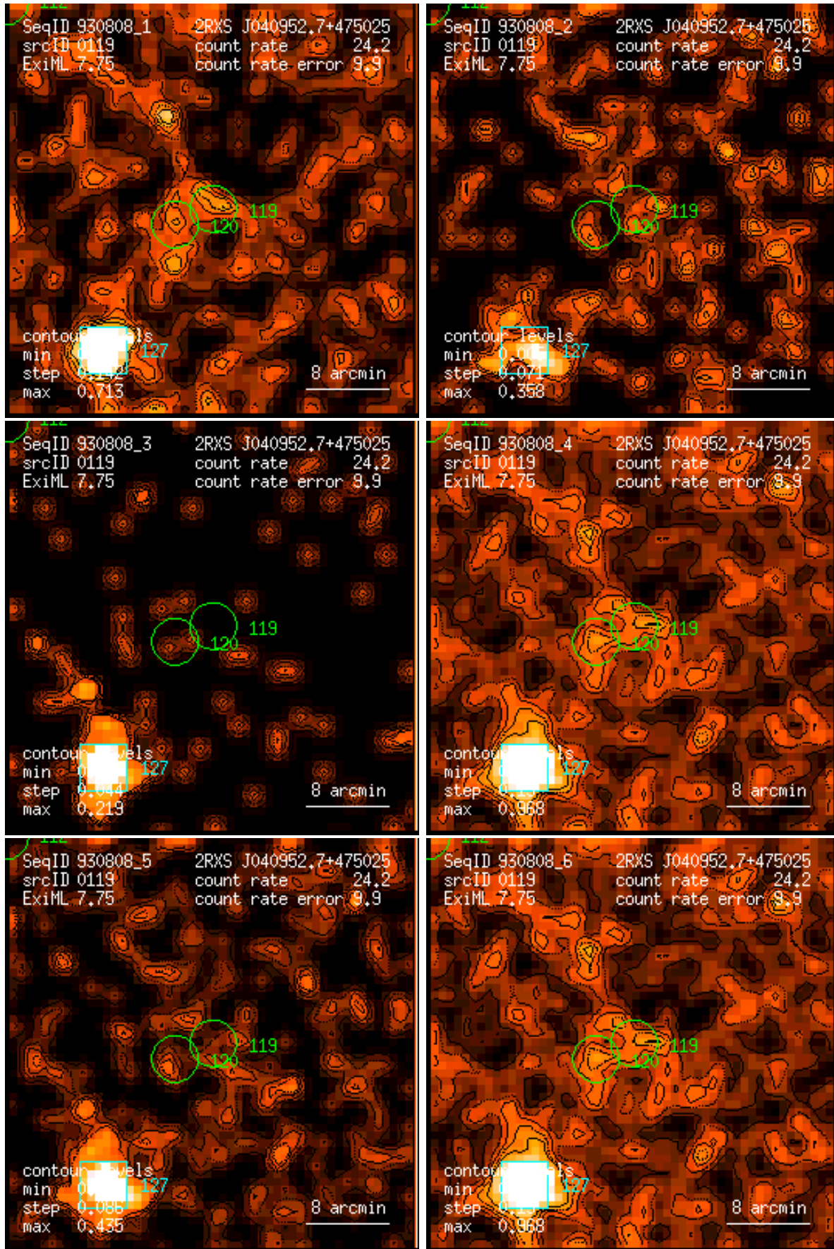
Figure 119: RASS 930808: detection 0119: band rate images, Gaussian filter: (1) PSPC channels 11 – 41, (2) 52 – 90, (3) 91 – 201, (4) 11 – 235, (5) 52 – 201, (6) 11 – 201. Broad band rates in counts/ks. Band rate contour levels in counts/ks/arcmin 2 .
