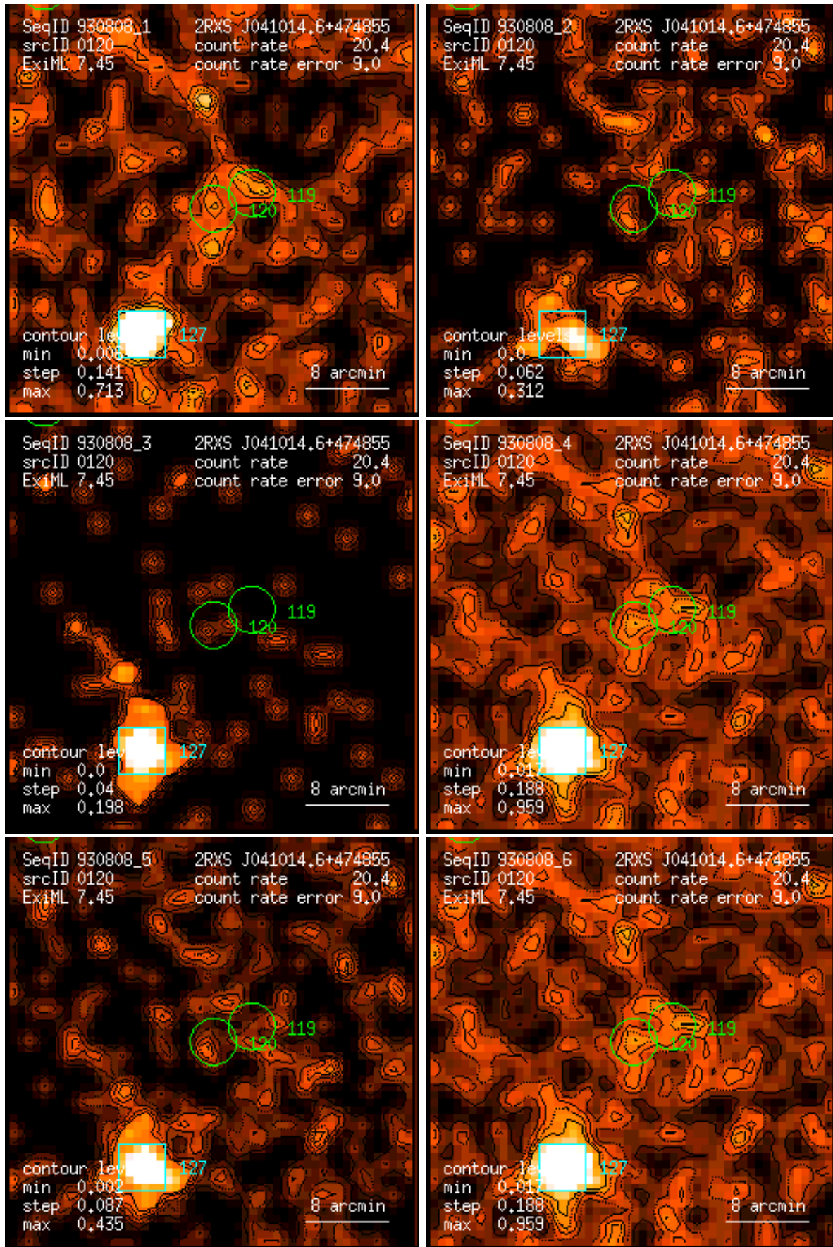
Figure 120: RASS 930808: detection 0120: band rate images, Gaussian filter: (1) PSPC channels 11 – 41, (2) 52 – 90, (3) 91 – 201, (4) 11 – 235, (5) 52 – 201, (6) 11 – 201. Broad band rates in counts/ks. Band rate contour levels in counts/ks/arcmin 2 .
