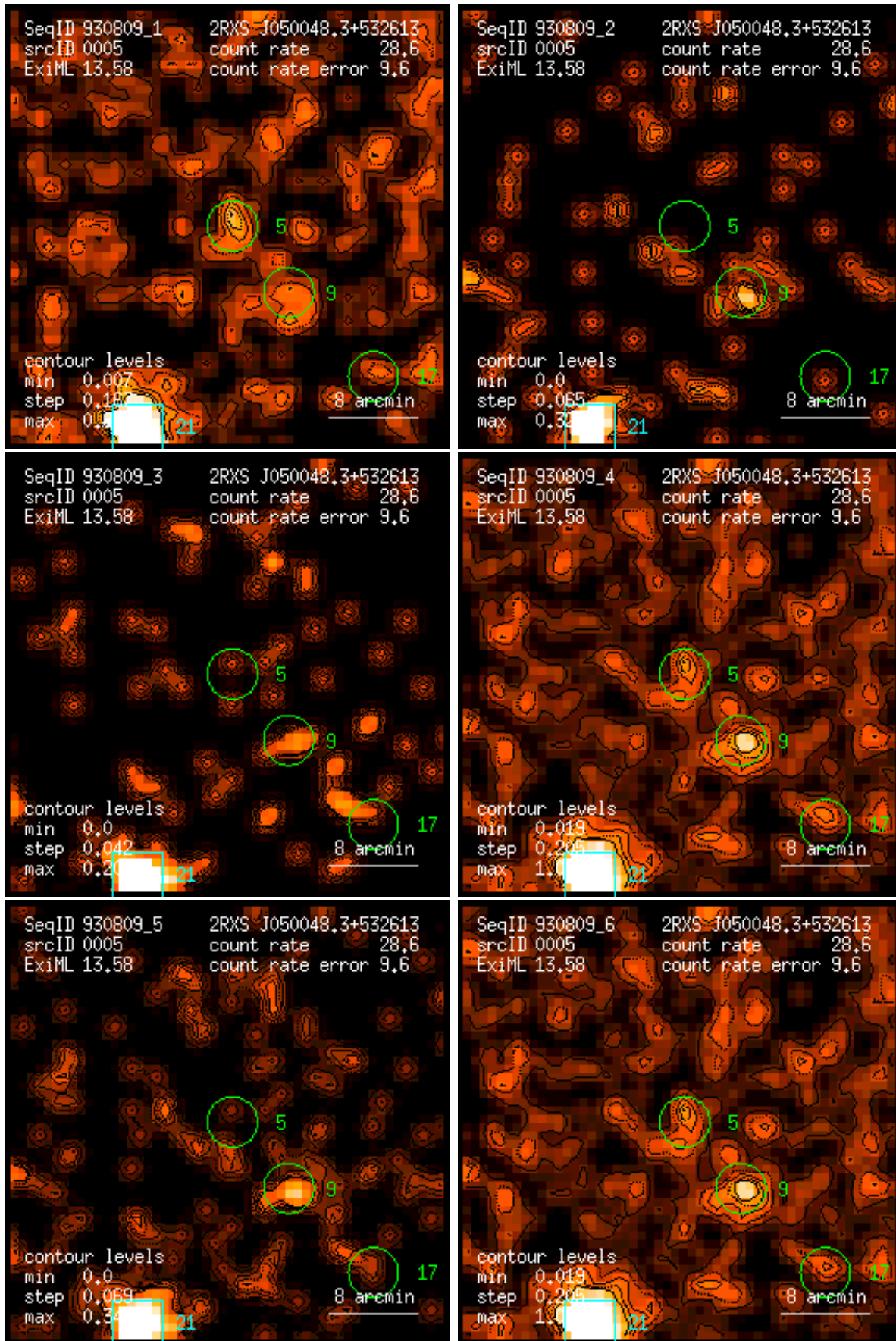
Figure 5: RASS 930809: detection 0005: band rate images, Gaussian filter: (1) PSPC channels 11 – 41, (2) 52 – 90, (3) 91 – 201, (4) 11 – 235, (5) 52 – 201, (6) 11 – 201. Broad band rates in counts/ks. Band rate contour levels in counts/ks/arcmin 2 .
