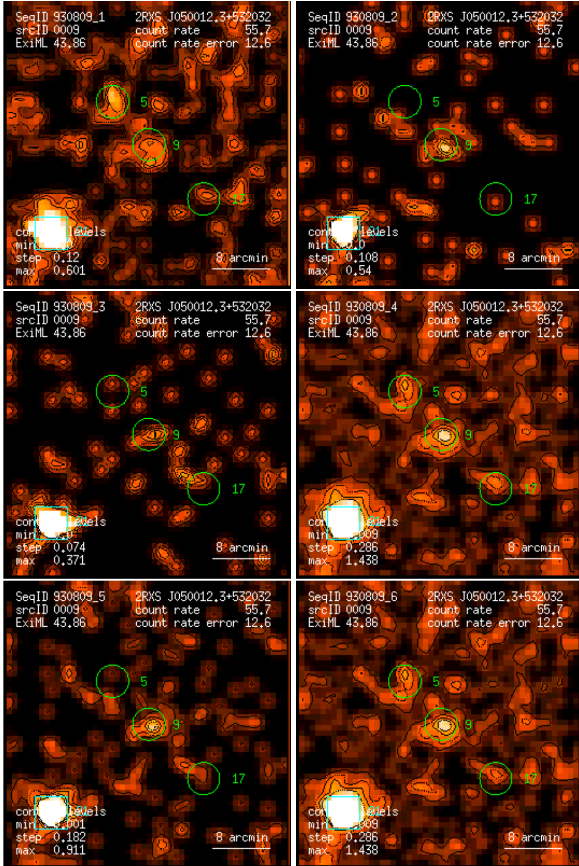
Figure 9: RASS 930809: detection 0009: band rate images, Gaussian filter: (1) PSPC channels 11 – 41, (2) 52 – 90, (3) 91 – 201, (4) 11 – 235, (5) 52 – 201, (6) 11 – 201. Broad band rates in counts/ks. Band rate contour levels in counts/ks/arcmin 2 .
