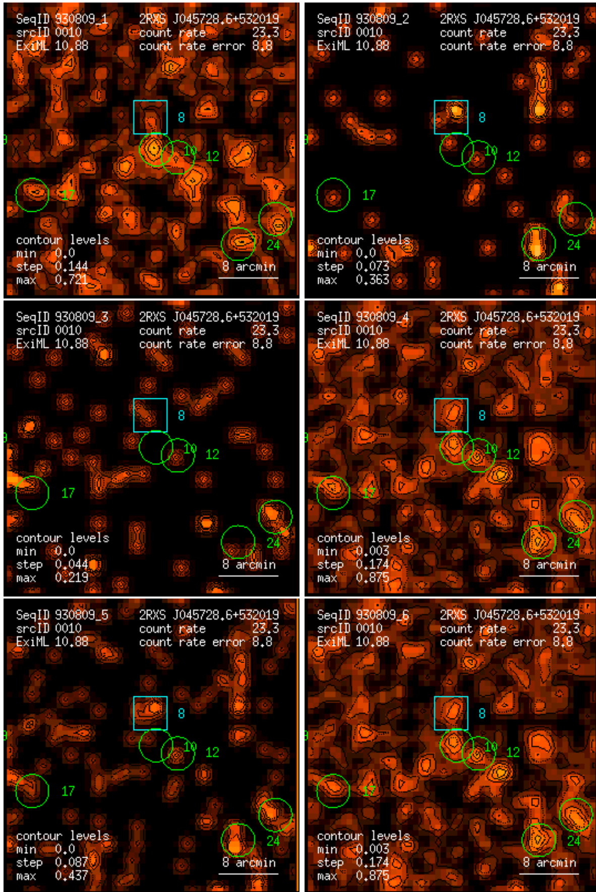
Figure 10: RASS 930809: detection 0010: band rate images, Gaussian filter: (1) PSPC channels 11 – 41, (2) 52 – 90, (3) 91 – 201, (4) 11 – 235, (5) 52 – 201, (6) 11 – 201. Broad band rates in counts/ks. Band rate contour levels in counts/ks/arcmin 2 .
