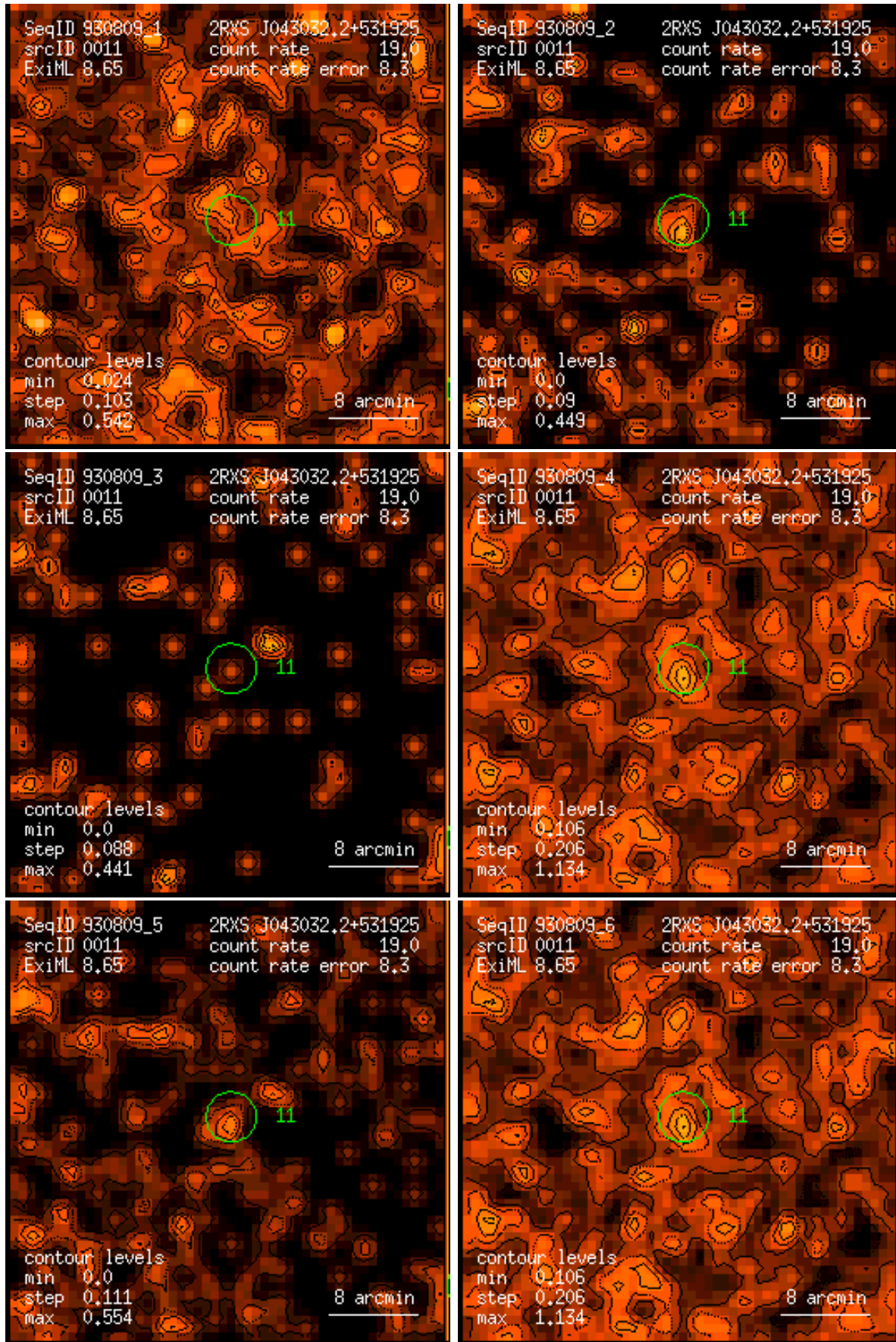
Figure 11: RASS 930809: detection 0011: band rate images, Gaussian filter: (1) PSPC channels 11 – 41, (2) 52 – 90, (3) 91 – 201, (4) 11 – 235, (5) 52 – 201, (6) 11 – 201. Broad band rates in counts/ks. Band rate contour levels in counts/ks/arcmin 2 .
