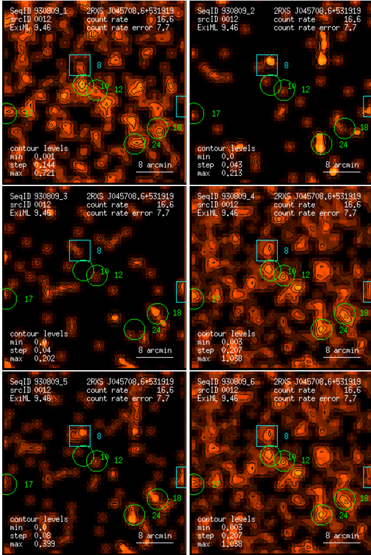
Figure 12: RASS 930809: detection 0012: band rate images, Gaussian filter: (1) PSPC channels 11 – 41, (2) 52 – 90, (3) 91 – 201, (4) 11 – 235, (5) 52 – 201, (6) 11 – 201. Broad band rates in counts/ks. Band rate contour levels in counts/ks/arcmin 2 .
