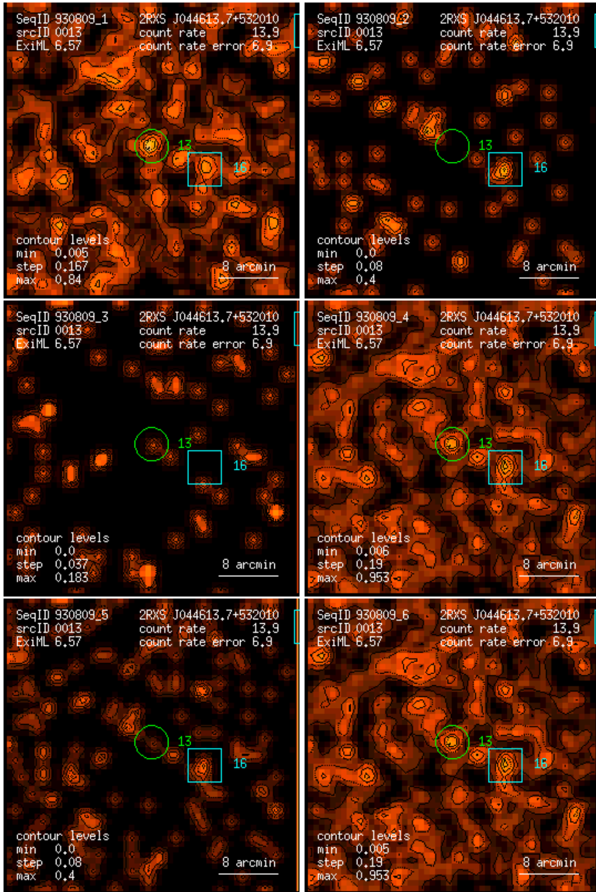
Figure 13: RASS 930809: detection 0013: band rate images, Gaussian filter: (1) PSPC channels 11 – 41, (2) 52 – 90, (3) 91 – 201, (4) 11 – 235, (5) 52 – 201, (6) 11 – 201. Broad band rates in counts/ks. Band rate contour levels in counts/ks/arcmin 2 .
