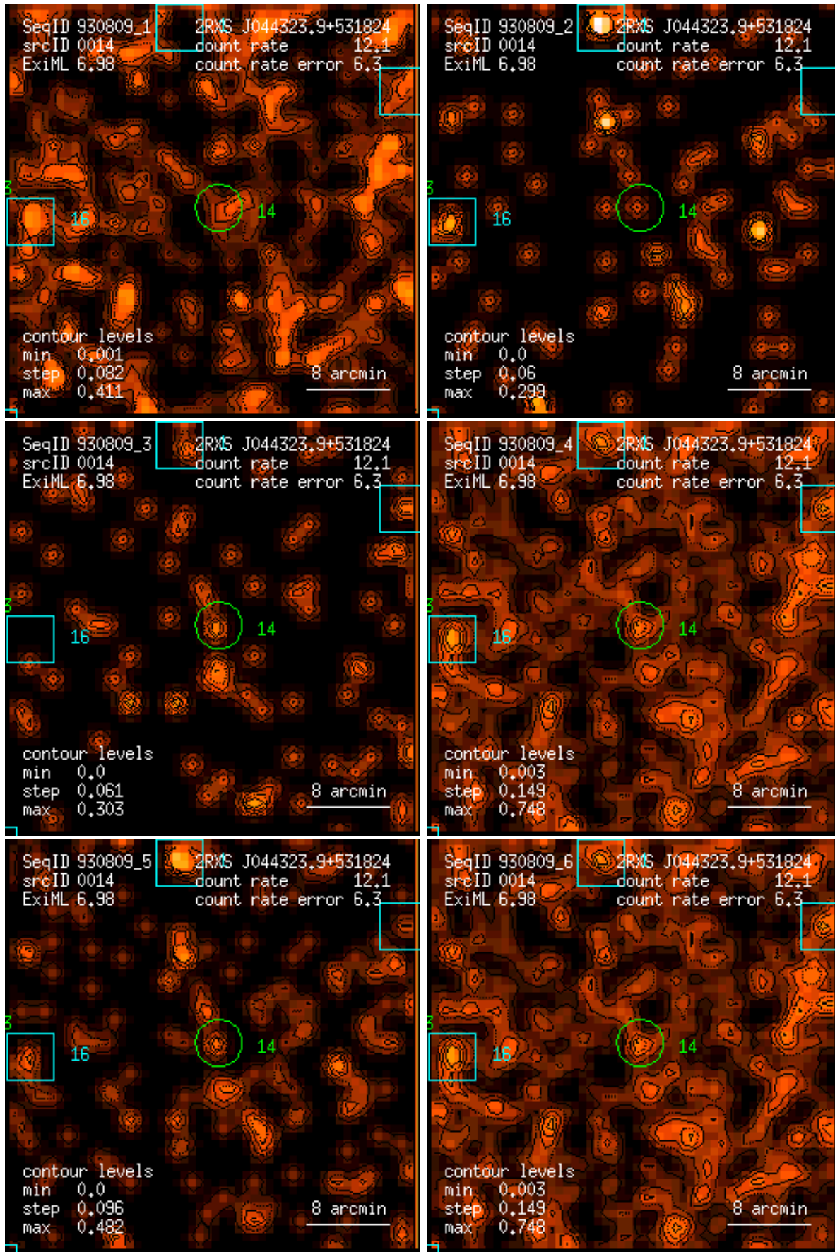
Figure 14: RASS 930809: detection 0014: band rate images, Gaussian filter: (1) PSPC channels 11 – 41, (2) 52 – 90, (3) 91 – 201, (4) 11 – 235, (5) 52 – 201, (6) 11 – 201. Broad band rates in counts/ks. Band rate contour levels in counts/ks/arcmin 2 .
