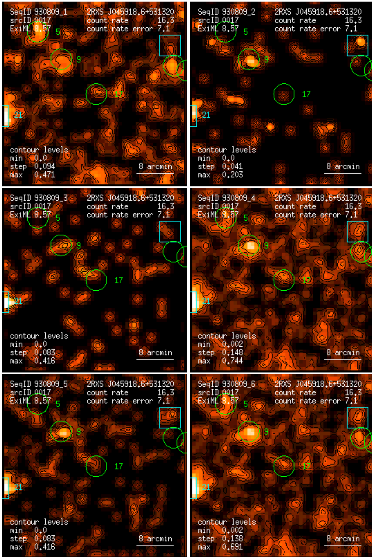
Figure 17: RASS 930809: detection 0017: band rate images, Gaussian filter: (1) PSPC channels 11 – 41, (2) 52 – 90, (3) 91 – 201, (4) 11 – 235, (5) 52 – 201, (6) 11 – 201. Broad band rates in counts/ks. Band rate contour levels in counts/ks/arcmin 2 .
