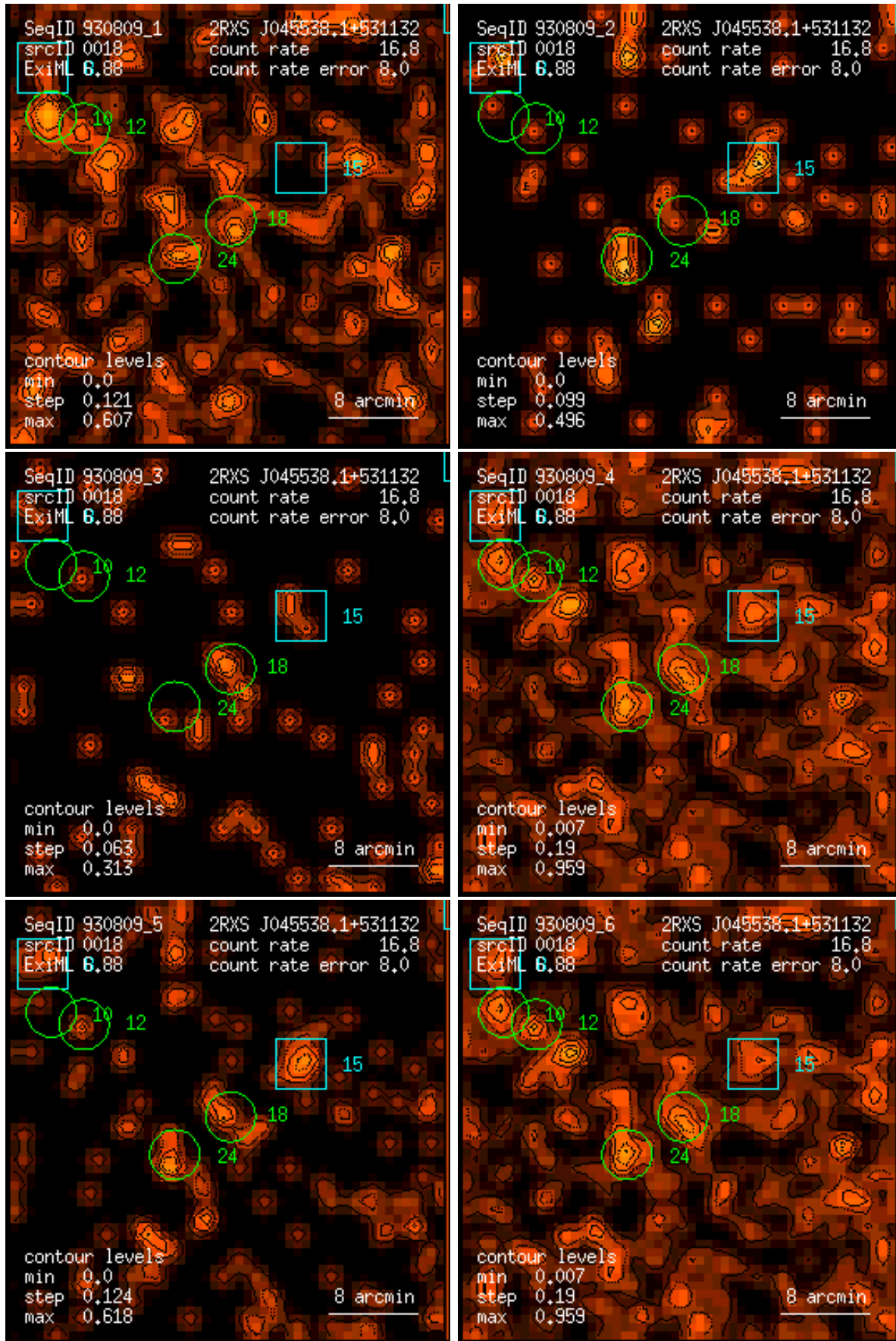
Figure 18: RASS 930809: detection 0018: band rate images, Gaussian filter: (1) PSPC channels 11 – 41, (2) 52 – 90, (3) 91 – 201, (4) 11 – 235, (5) 52 – 201, (6) 11 – 201. Broad band rates in counts/ks. Band rate contour levels in counts/ks/arcmin 2 .
