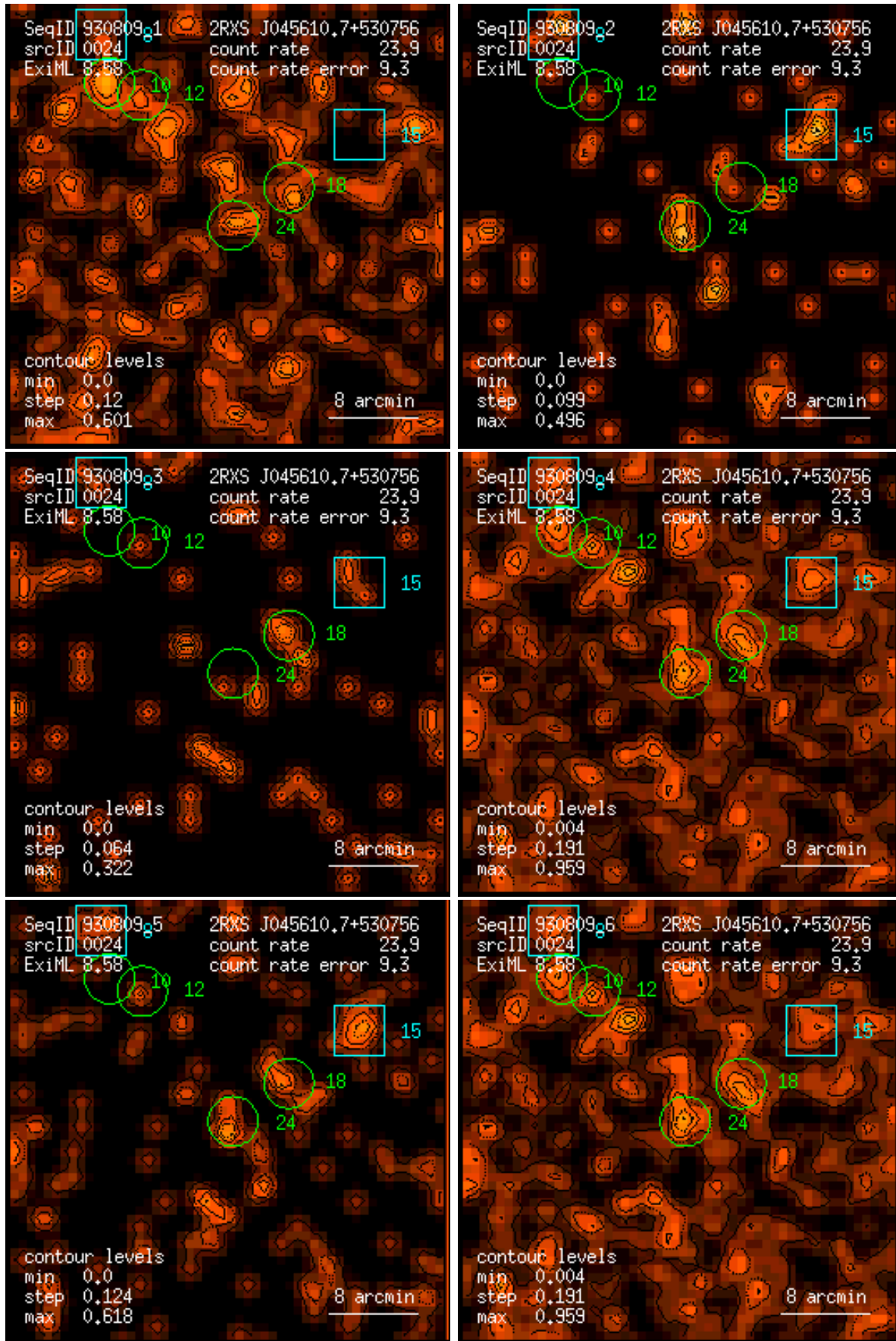
Figure 24: RASS 930809: detection 0024: band rate images, Gaussian filter: (1) PSPC channels 11 – 41, (2) 52 – 90, (3) 91 – 201, (4) 11 – 235, (5) 52 – 201, (6) 11 – 201. Broad band rates in counts/ks. Band rate contour levels in counts/ks/arcmin 2 .
