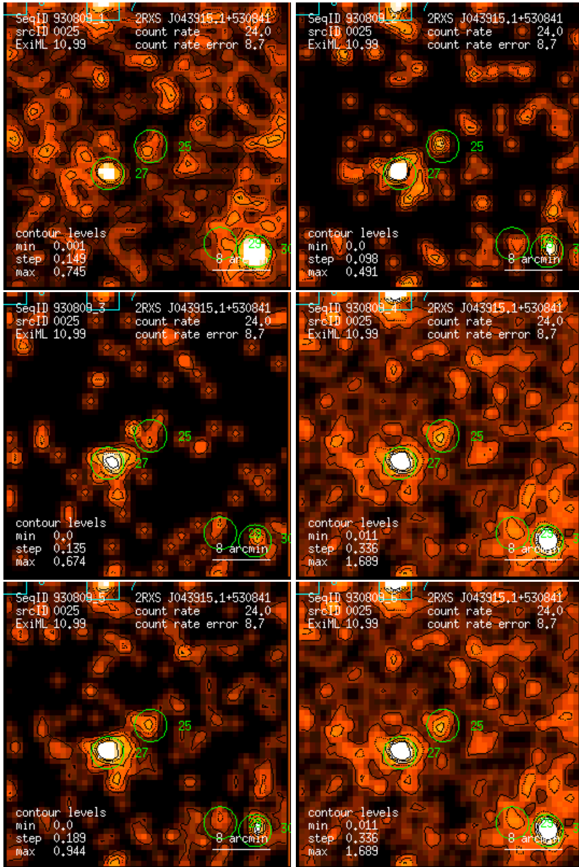
Figure 25: RASS 930809: detection 0025: band rate images, Gaussian filter: (1) PSPC channels 11 – 41, (2) 52 – 90, (3) 91 – 201, (4) 11 – 235, (5) 52 – 201, (6) 11 – 201. Broad band rates in counts/ks. Band rate contour levels in counts/ks/arcmin 2 .
