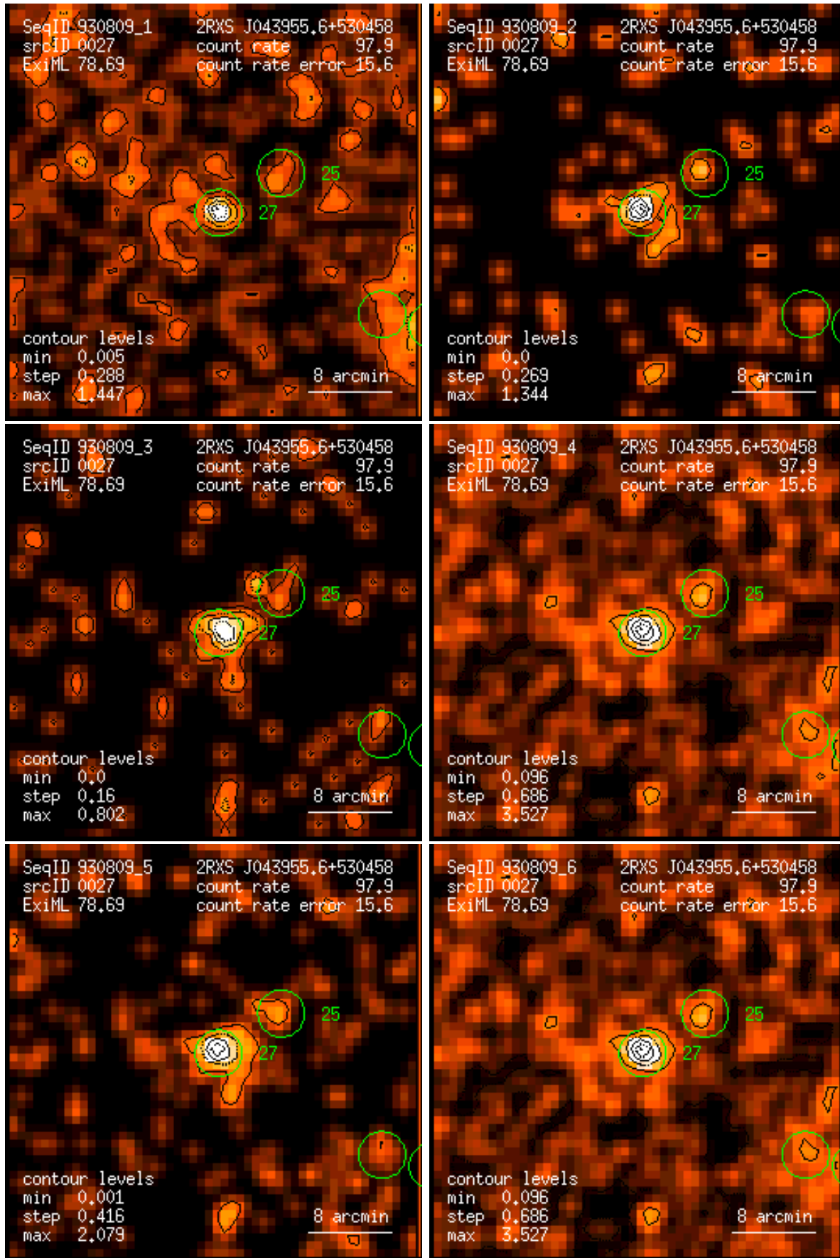
Figure 27: RASS 930809: detection 0027: band rate images, Gaussian filter: (1) PSPC channels 11 – 41, (2) 52 – 90, (3) 91 – 201, (4) 11 – 235, (5) 52 – 201, (6) 11 – 201. Broad band rates in counts/ks. Band rate contour levels in counts/ks/arcmin 2 .
