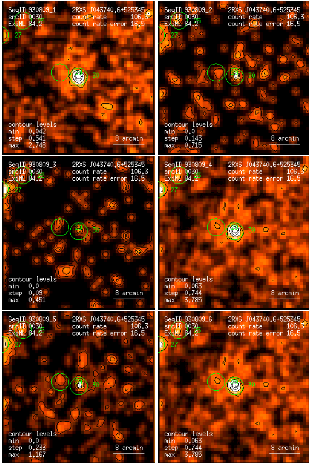
Figure 30: RASS 930809: detection 0030: band rate images, Gaussian filter: (1) PSPC channels 11 – 41, (2) 52 – 90, (3) 91 – 201, (4) 11 – 235, (5) 52 – 201, (6) 11 – 201. Broad band rates in counts/ks. Band rate contour levels in counts/ks/arcmin 2 .
