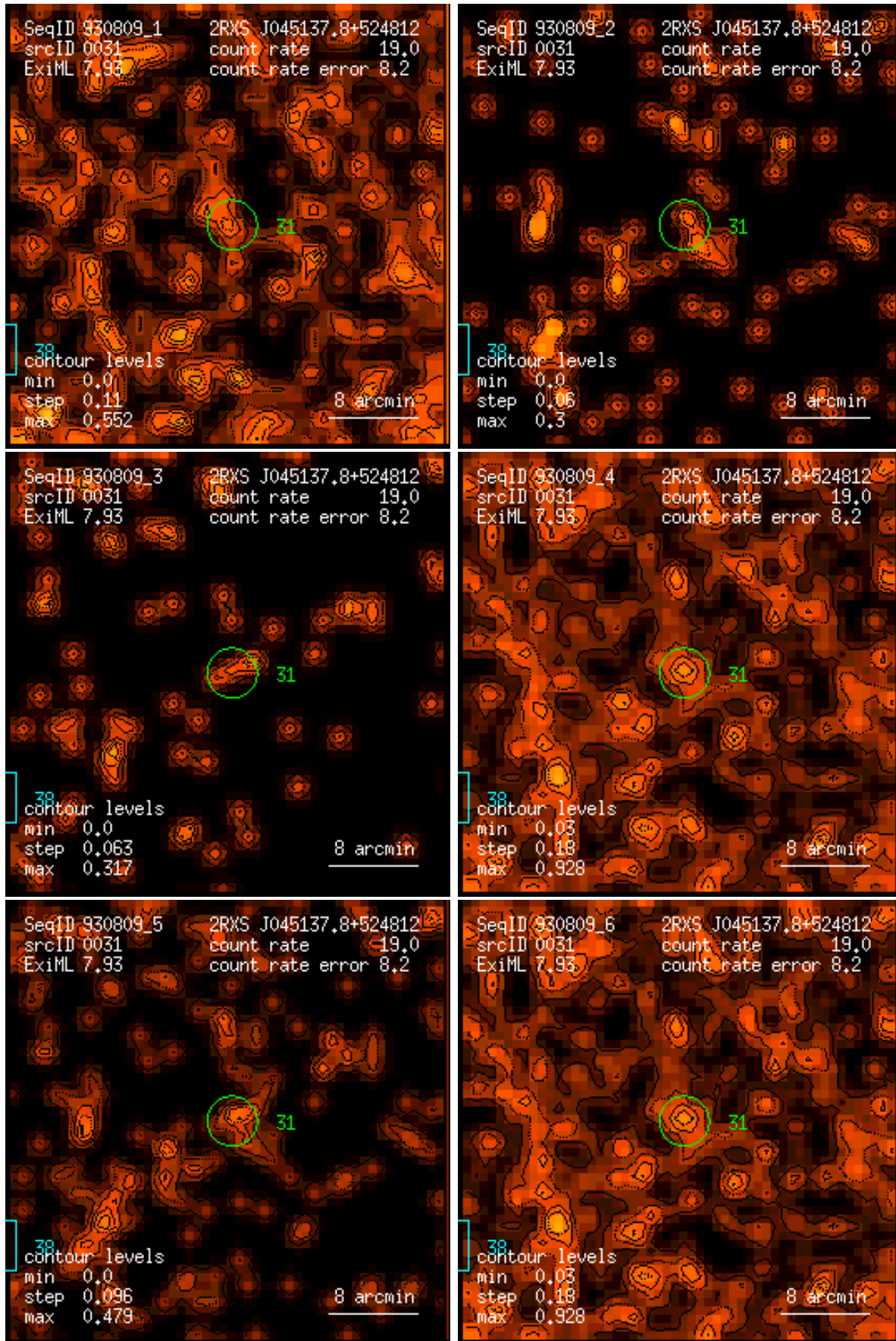
Figure 31: RASS 930809: detection 0031: band rate images, Gaussian filter: (1) PSPC channels 11 – 41, (2) 52 – 90, (3) 91 – 201, (4) 11 – 235, (5) 52 – 201, (6) 11 – 201. Broad band rates in counts/ks. Band rate contour levels in counts/ks/arcmin 2 .
