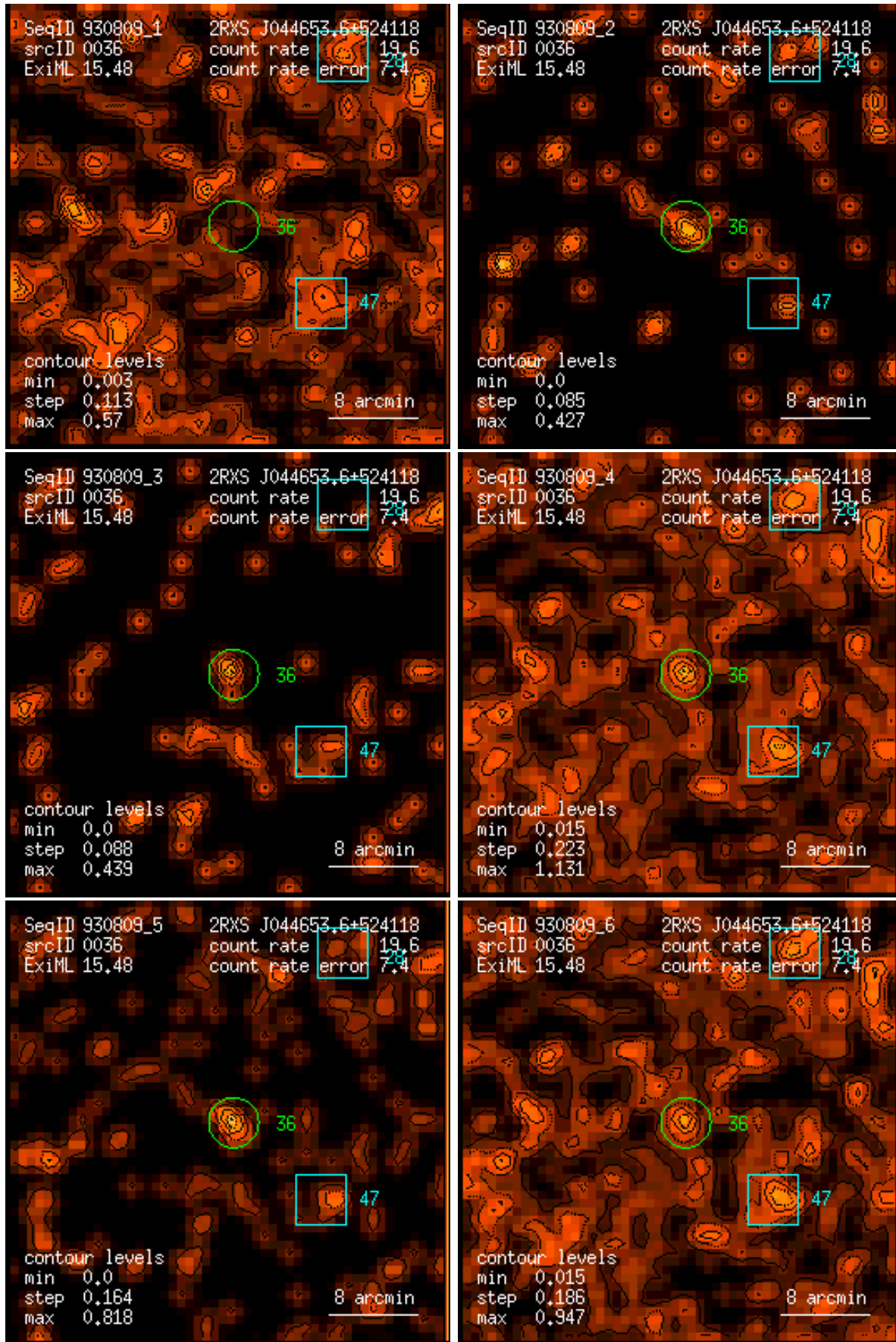
Figure 36: RASS 930809: detection 0036: band rate images, Gaussian filter: (1) PSPC channels 11 – 41, (2) 52 – 90, (3) 91 – 201, (4) 11 – 235, (5) 52 – 201, (6) 11 – 201. Broad band rates in counts/ks. Band rate contour levels in counts/ks/arcmin 2 .
