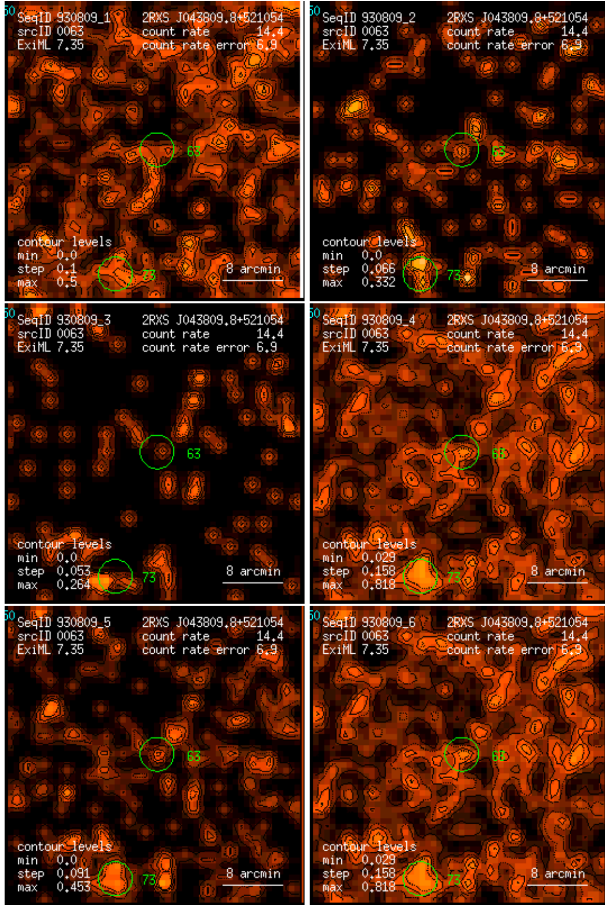
Figure 63: RASS 930809: detection 0063: band rate images, Gaussian filter: (1) PSPC channels 11 – 41, (2) 52 – 90, (3) 91 – 201, (4) 11 – 235, (5) 52 – 201, (6) 11 – 201. Broad band rates in counts/ks. Band rate contour levels in counts/ks/arcmin 2 .
