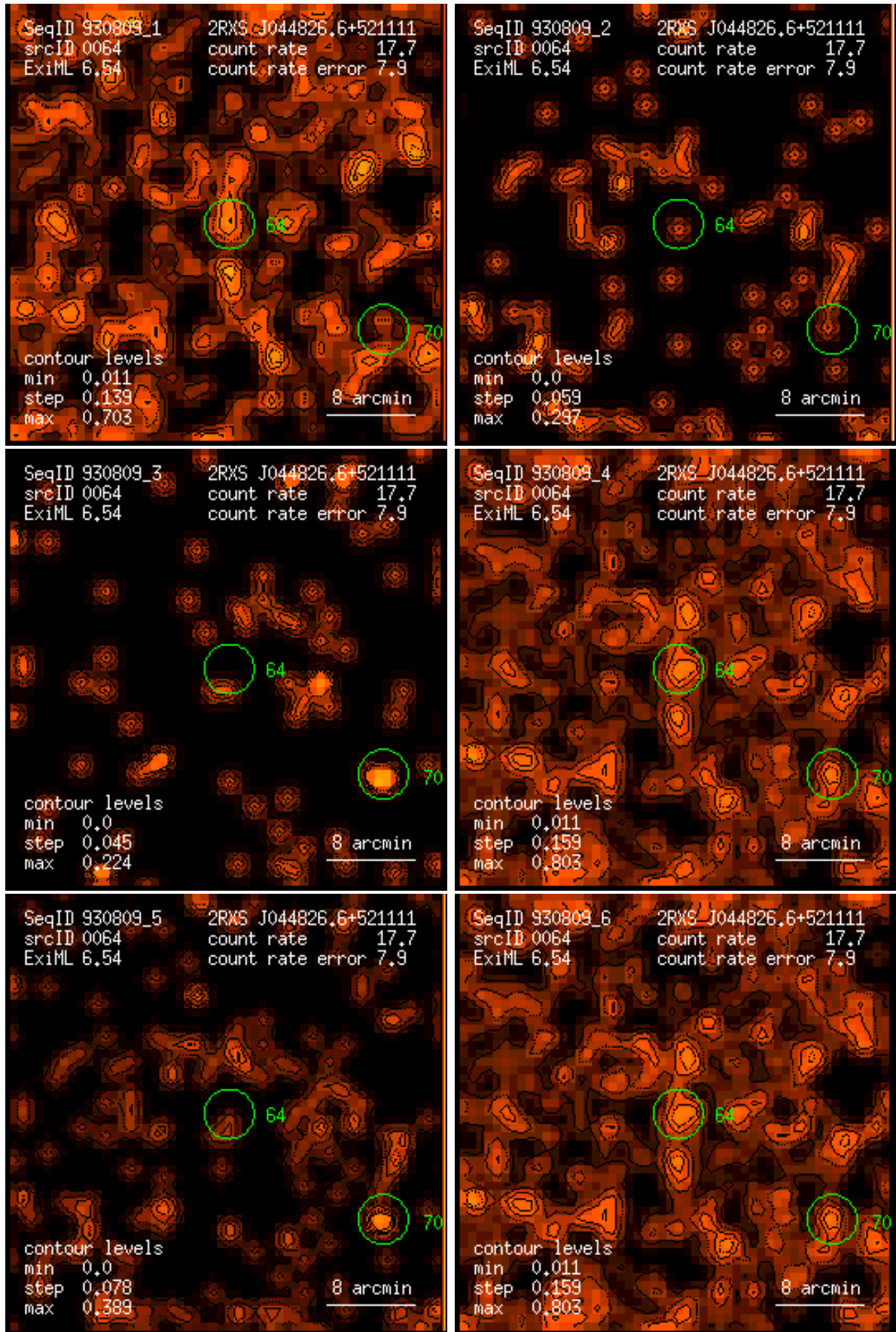
Figure 64: RASS 930809: detection 0064: band rate images, Gaussian filter: (1) PSPC channels 11 – 41, (2) 52 – 90, (3) 91 – 201, (4) 11 – 235, (5) 52 – 201, (6) 11 – 201. Broad band rates in counts/ks. Band rate contour levels in counts/ks/arcmin 2 .
