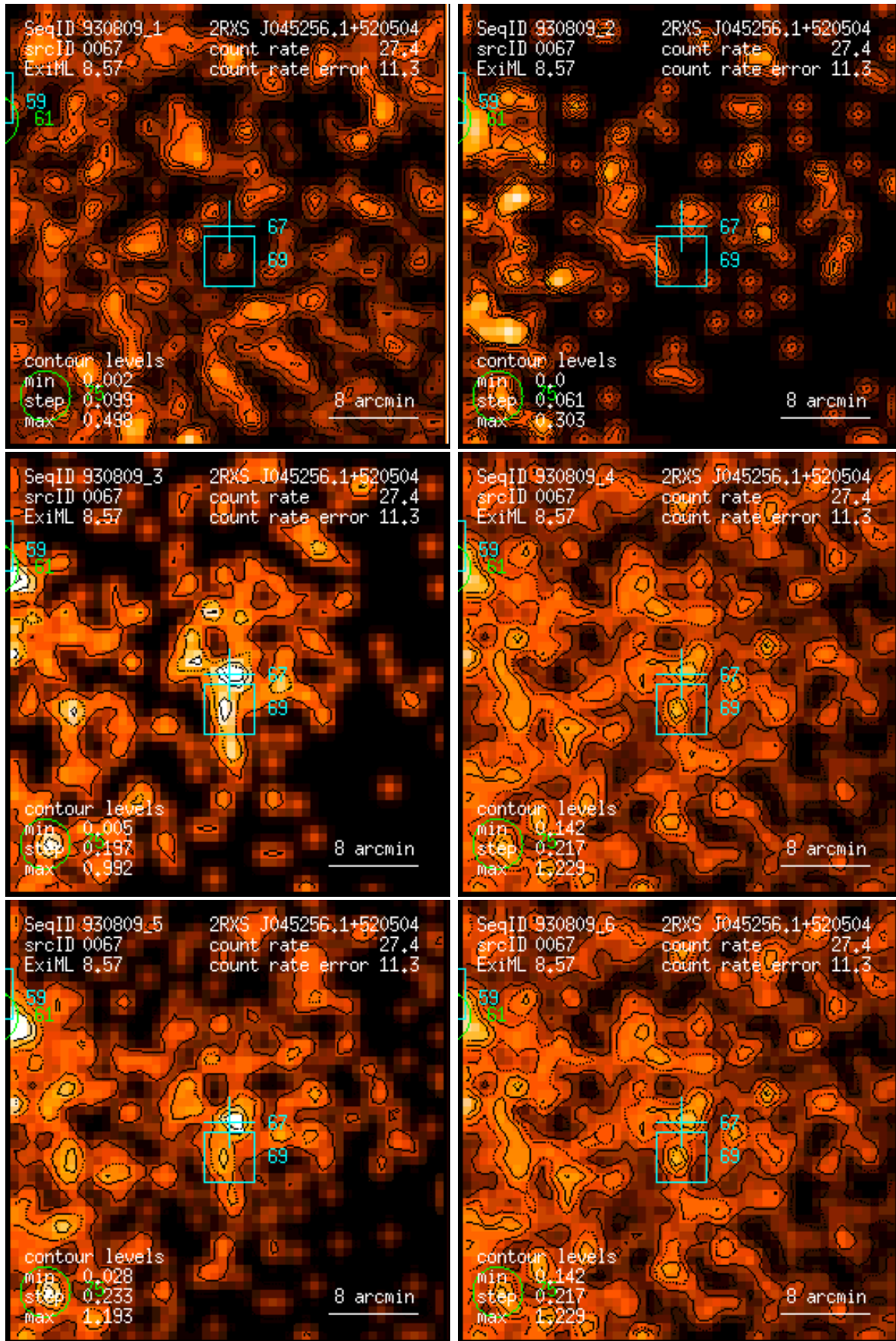
Figure 67: RASS 930809: detection 0067: band rate images, Gaussian filter: (1) PSPC channels 11 – 41, (2) 52 – 90, (3) 91 – 201, (4) 11 – 235, (5) 52 – 201, (6) 11 – 201. Broad band rates in counts/ks. Band rate contour levels in counts/ks/arcmin 2 .
