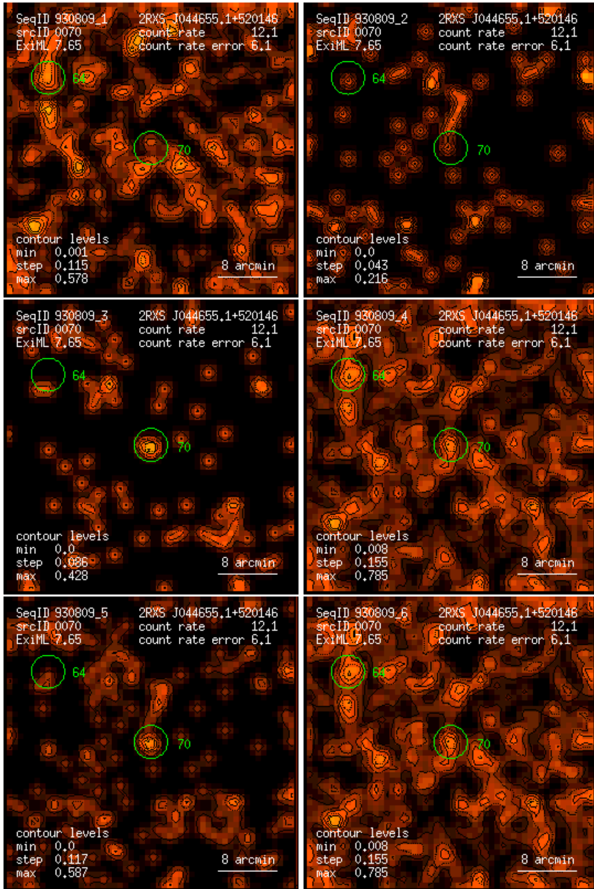
Figure 70: RASS 930809: detection 0070: band rate images, Gaussian filter: (1) PSPC channels 11 – 41, (2) 52 – 90, (3) 91 – 201, (4) 11 – 235, (5) 52 – 201, (6) 11 – 201. Broad band rates in counts/ks. Band rate contour levels in counts/ks/arcmin 2 .
