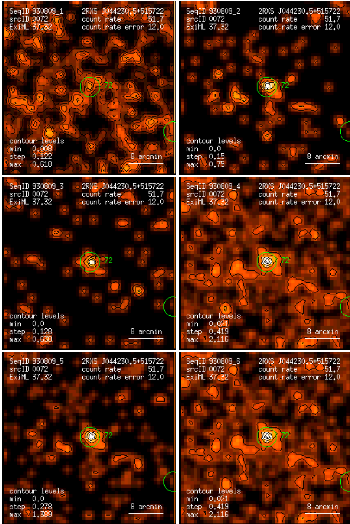
Figure 72: RASS 930809: detection 0072: band rate images, Gaussian filter: (1) PSPC channels 11 – 41, (2) 52 – 90, (3) 91 – 201, (4) 11 – 235, (5) 52 – 201, (6) 11 – 201. Broad band rates in counts/ks. Band rate contour levels in counts/ks/arcmin 2 .
