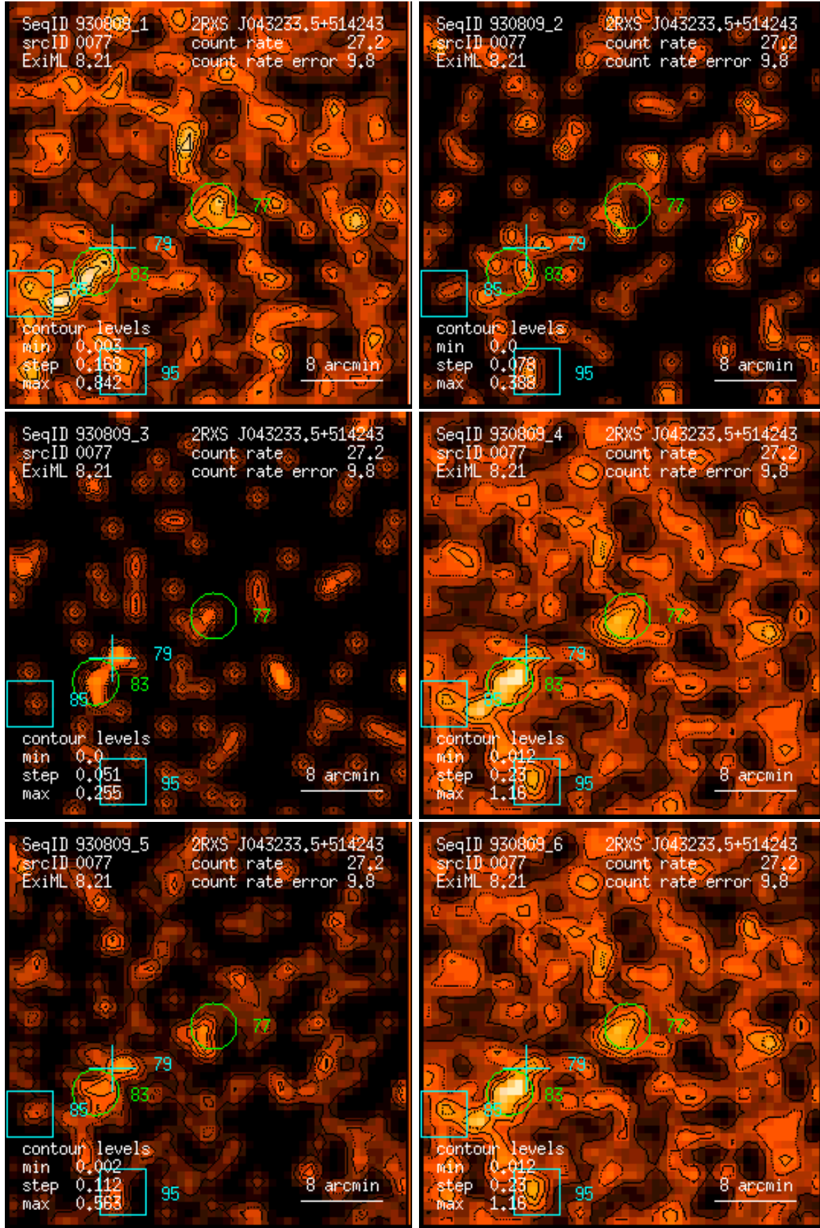
Figure 77: RASS 930809: detection 0077: band rate images, Gaussian filter: (1) PSPC channels 11 – 41, (2) 52 – 90, (3) 91 – 201, (4) 11 – 235, (5) 52 – 201, (6) 11 – 201. Broad band rates in counts/ks. Band rate contour levels in counts/ks/arcmin 2 .
