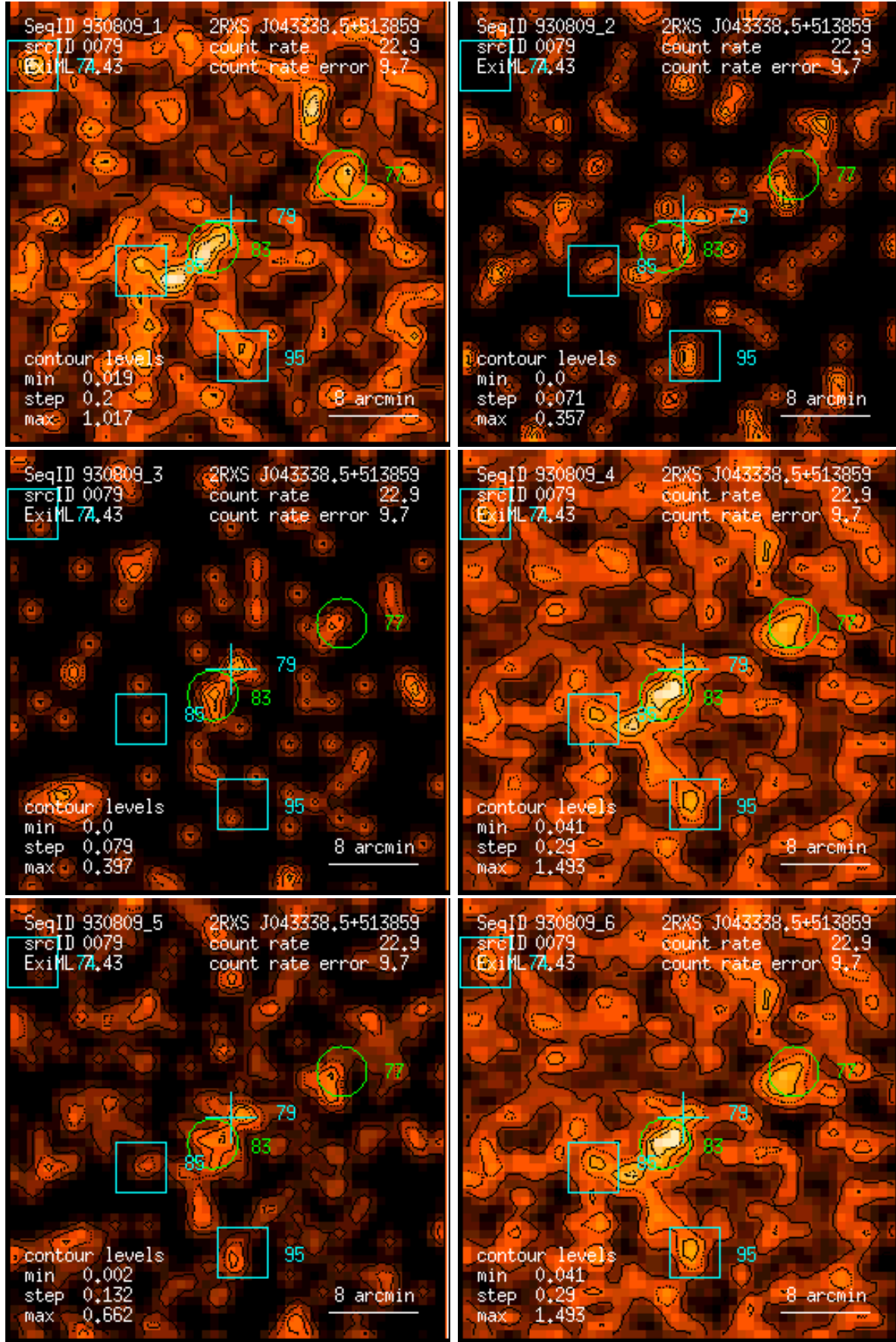
Figure 79: RASS 930809: detection 0079: band rate images, Gaussian filter: (1) PSPC channels 11 – 41, (2) 52 – 90, (3) 91 – 201, (4) 11 – 235, (5) 52 – 201, (6) 11 – 201. Broad band rates in counts/ks. Band rate contour levels in counts/ks/arcmin 2 .
