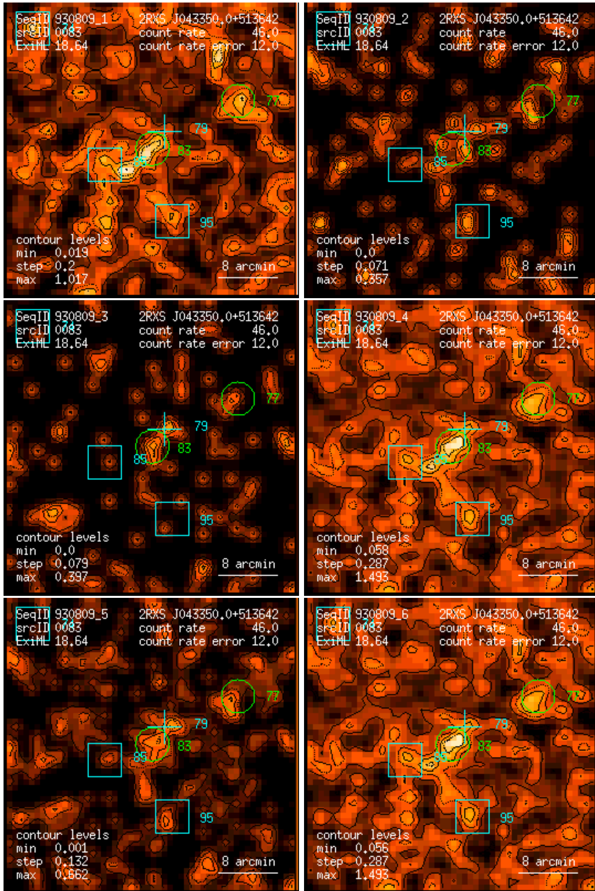
Figure 83: RASS 930809: detection 0083: band rate images, Gaussian filter: (1) PSPC channels 11 – 41, (2) 52 – 90, (3) 91 – 201, (4) 11 – 235, (5) 52 – 201, (6) 11 – 201. Broad band rates in counts/ks. Band rate contour levels in counts/ks/arcmin 2 .
