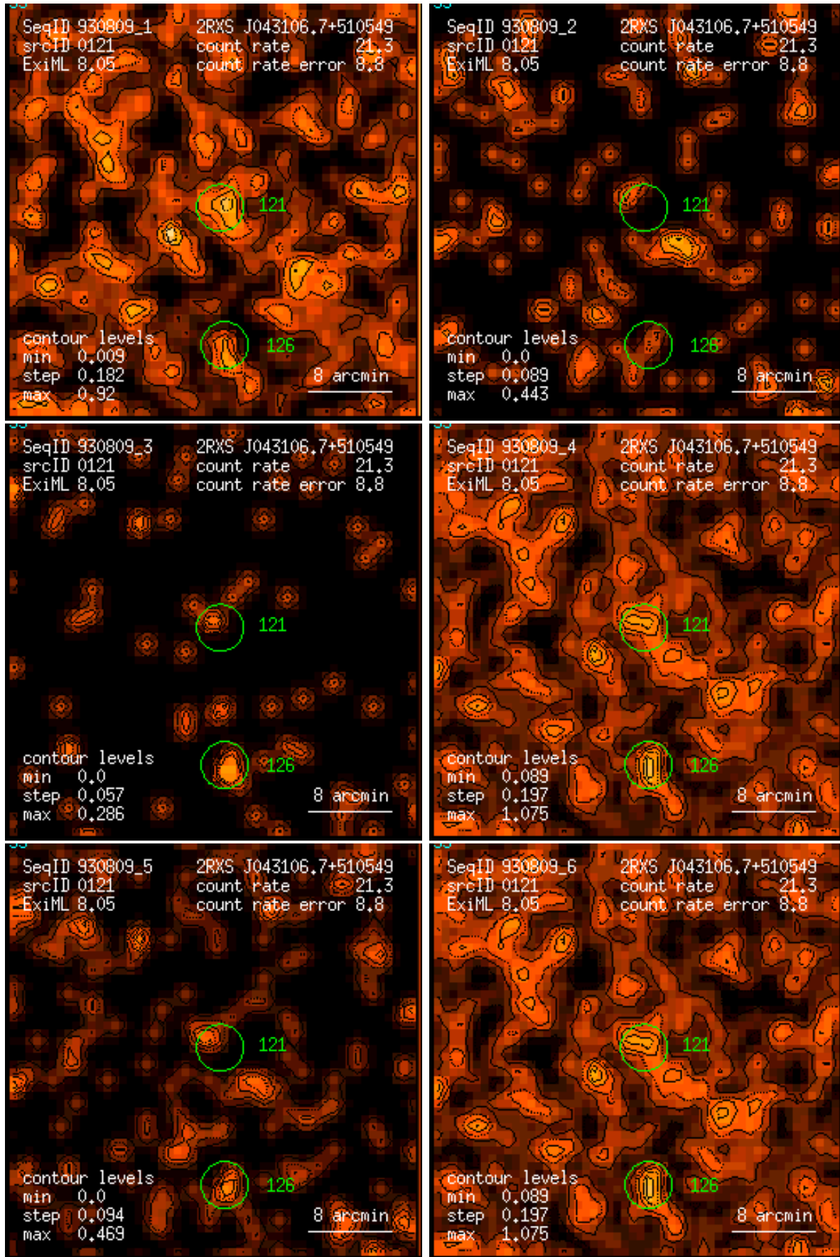
Figure 121: RASS 930809: detection 0121: band rate images, Gaussian filter: (1) PSPC channels 11 – 41, (2) 52 – 90, (3) 91 – 201, (4) 11 – 235, (5) 52 – 201, (6) 11 – 201. Broad band rates in counts/ks. Band rate contour levels in counts/ks/arcmin 2 .
