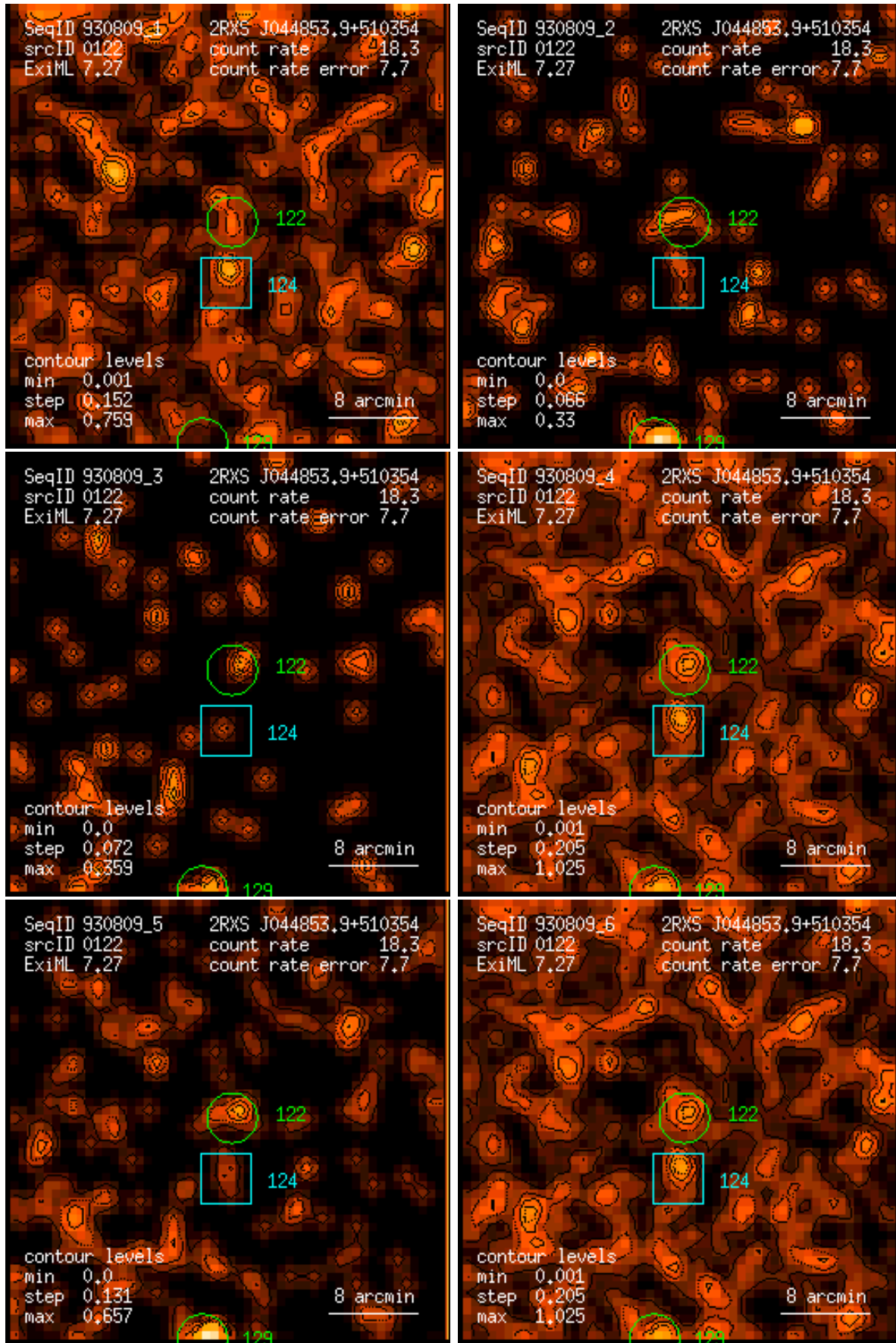
Figure 122: RASS 930809: detection 0122: band rate images, Gaussian filter: (1) PSPC channels 11 – 41, (2) 52 – 90, (3) 91 – 201, (4) 11 – 235, (5) 52 – 201, (6) 11 – 201. Broad band rates in counts/ks. Band rate contour levels in counts/ks/arcmin 2 .
