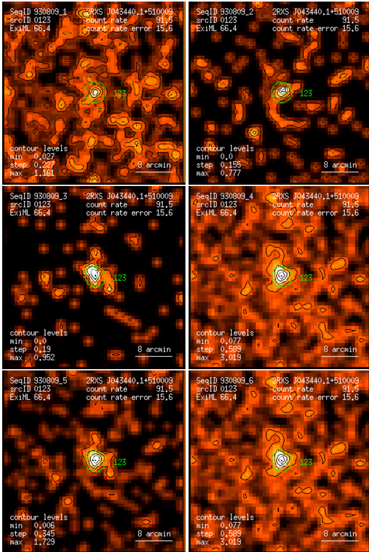
Figure 123: RASS 930809: detection 0123: band rate images, Gaussian filter: (1) PSPC channels 11 – 41, (2) 52 – 90, (3) 91 – 201, (4) 11 – 235, (5) 52 – 201, (6) 11 – 201. Broad band rates in counts/ks. Band rate contour levels in counts/ks/arcmin 2 .
