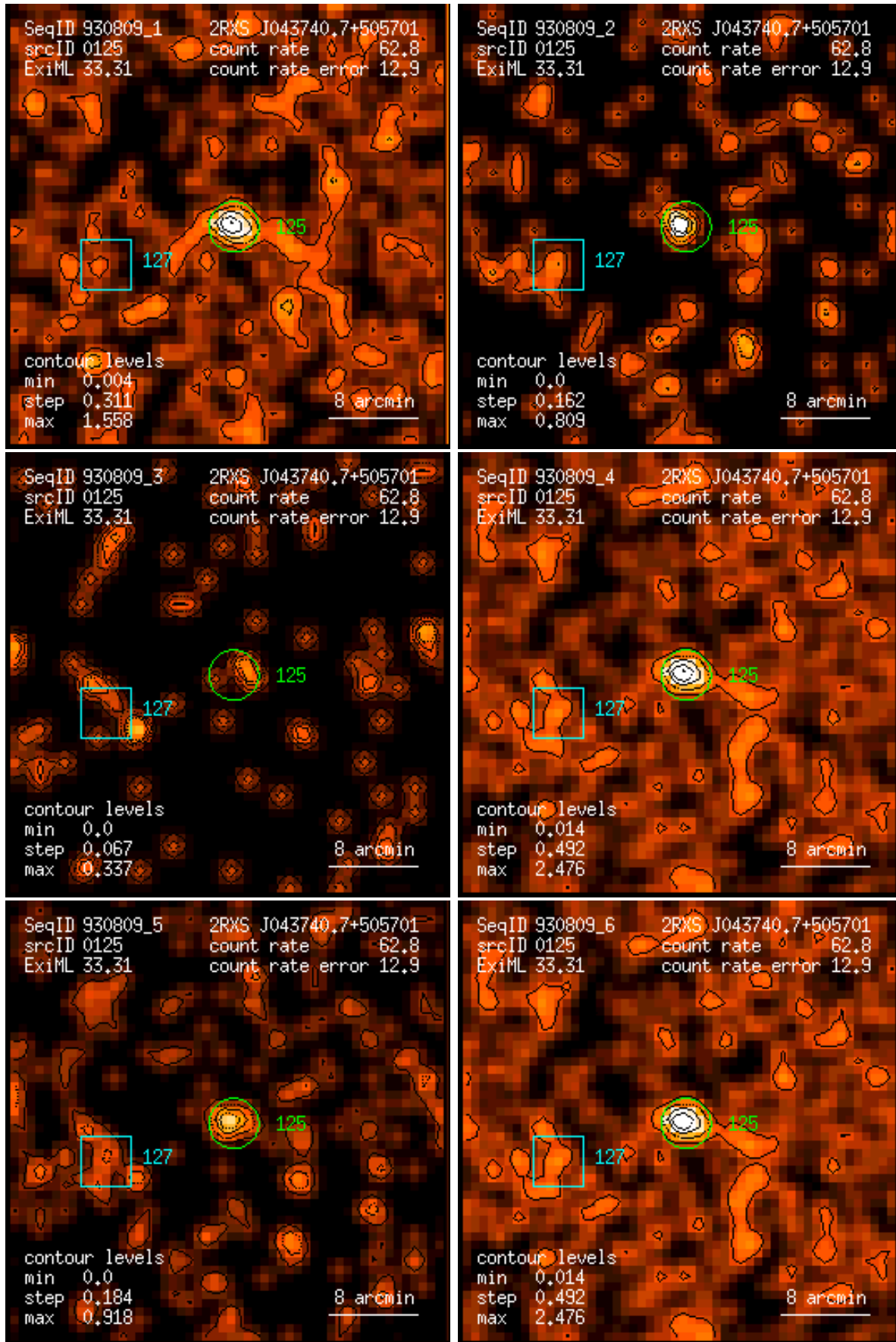
Figure 125: RASS 930809: detection 0125: band rate images, Gaussian filter: (1) PSPC channels 11 – 41, (2) 52 – 90, (3) 91 – 201, (4) 11 – 235, (5) 52 – 201, (6) 11 – 201. Broad band rates in counts/ks. Band rate contour levels in counts/ks/arcmin 2 .
