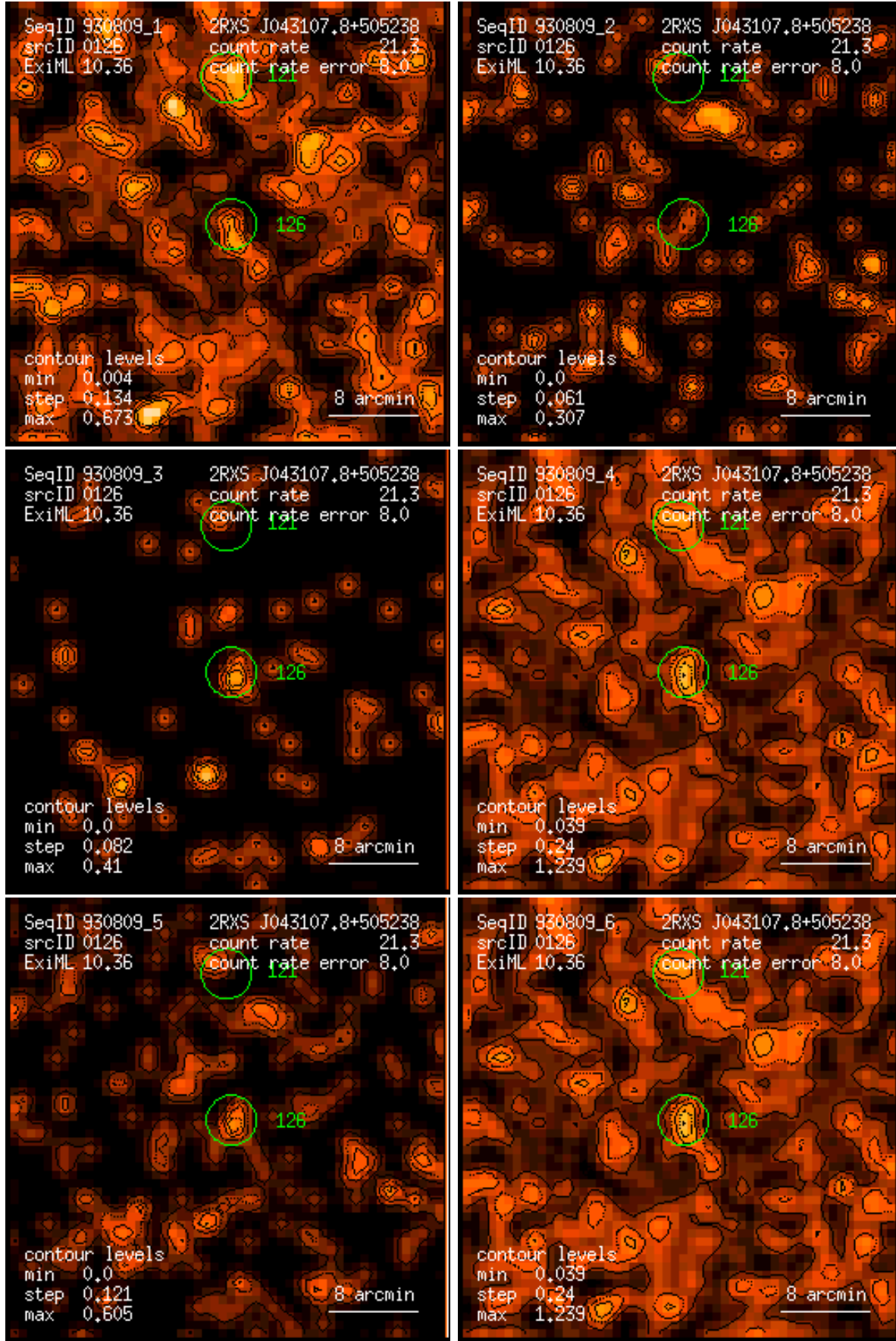
Figure 126: RASS 930809: detection 0126: band rate images, Gaussian filter: (1) PSPC channels 11 – 41, (2) 52 – 90, (3) 91 – 201, (4) 11 – 235, (5) 52 – 201, (6) 11 – 201. Broad band rates in counts/ks. Band rate contour levels in counts/ks/arcmin 2 .
