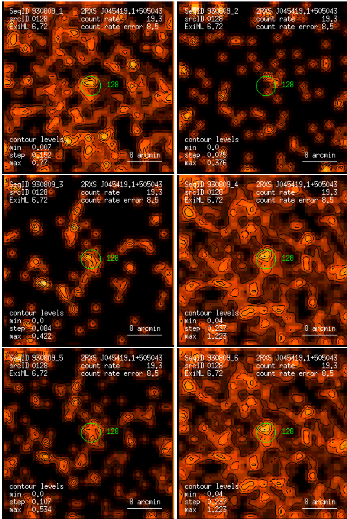
Figure 128: RASS 930809: detection 0128: band rate images, Gaussian filter: (1) PSPC channels 11 – 41, (2) 52 – 90, (3) 91 – 201, (4) 11 – 235, (5) 52 – 201, (6) 11 – 201. Broad band rates in counts/ks. Band rate contour levels in counts/ks/arcmin 2 .
