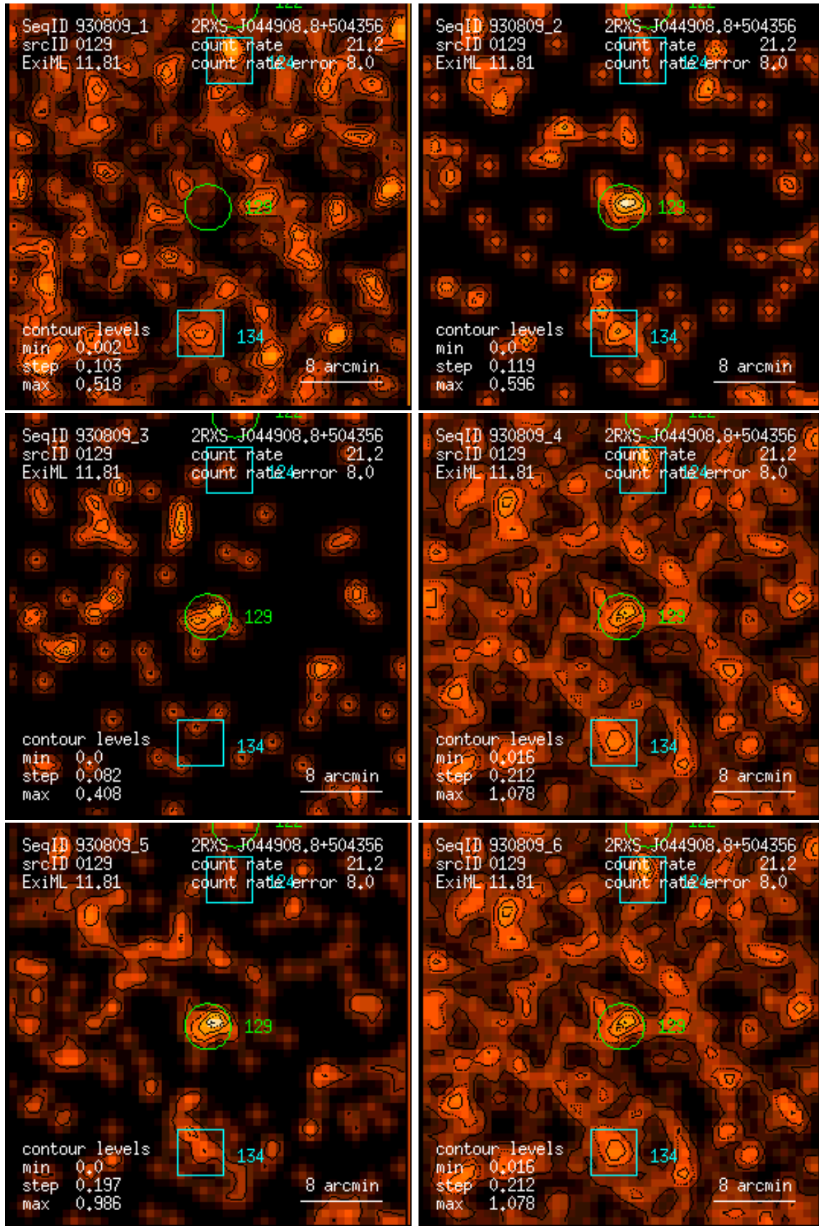
Figure 129: RASS 930809: detection 0129: band rate images, Gaussian filter: (1) PSPC channels 11 – 41, (2) 52 – 90, (3) 91 – 201, (4) 11 – 235, (5) 52 – 201, (6) 11 – 201. Broad band rates in counts/ks. Band rate contour levels in counts/ks/arcmin 2 .
