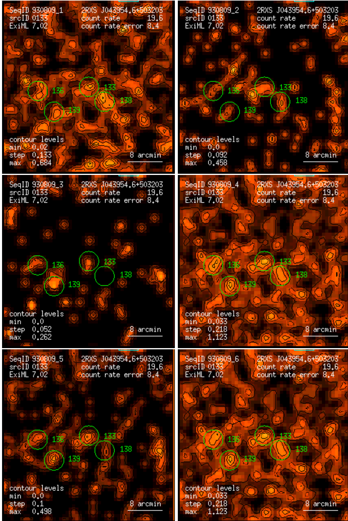
Figure 133: RASS 930809: detection 0133: band rate images, Gaussian filter: (1) PSPC channels 11 – 41, (2) 52 – 90, (3) 91 – 201, (4) 11 – 235, (5) 52 – 201, (6) 11 – 201. Broad band rates in counts/ks. Band rate contour levels in counts/ks/arcmin 2 .
