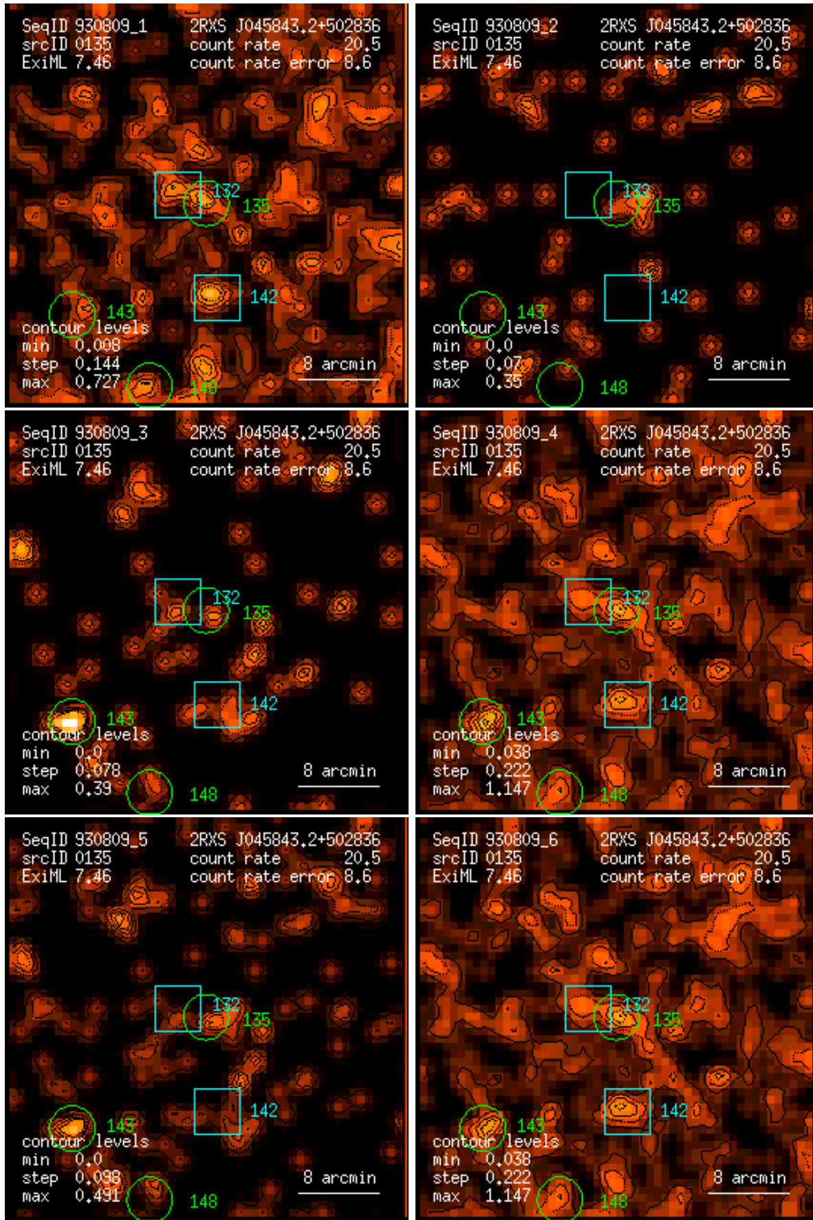
Figure 135: RASS 930809: detection 0135: band rate images, Gaussian filter: (1) PSPC channels 11 – 41, (2) 52 – 90, (3) 91 – 201, (4) 11 – 235, (5) 52 – 201, (6) 11 – 201. Broad band rates in counts/ks. Band rate contour levels in counts/ks/arcmin 2 .
