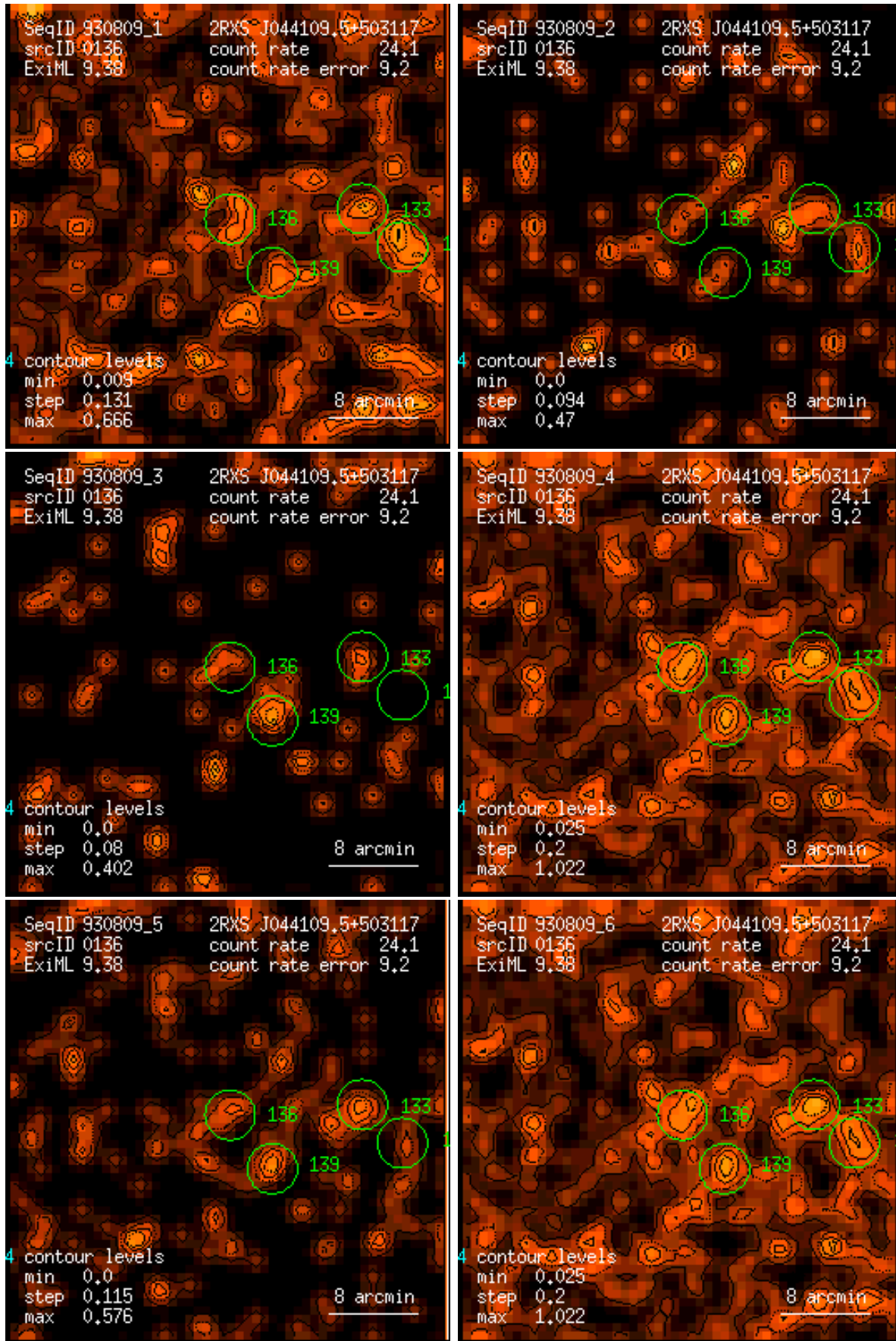
Figure 136: RASS 930809: detection 0136: band rate images, Gaussian filter: (1) PSPC channels 11 – 41, (2) 52 – 90, (3) 91 – 201, (4) 11 – 235, (5) 52 – 201, (6) 11 – 201. Broad band rates in counts/ks. Band rate contour levels in counts/ks/arcmin 2 .
