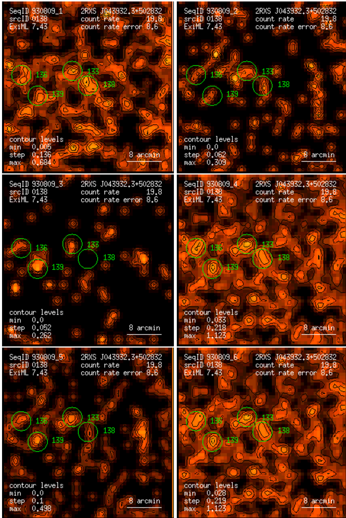
Figure 138: RASS 930809: detection 0138: band rate images, Gaussian filter: (1) PSPC channels 11 – 41, (2) 52 – 90, (3) 91 – 201, (4) 11 – 235, (5) 52 – 201, (6) 11 – 201. Broad band rates in counts/ks. Band rate contour levels in counts/ks/arcmin 2 .
