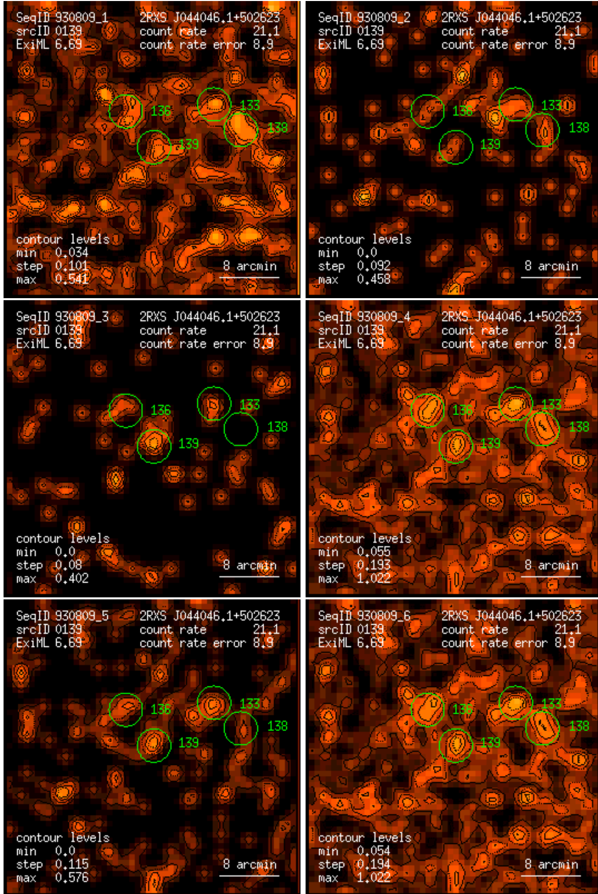
Figure 139: RASS 930809: detection 0139: band rate images, Gaussian filter: (1) PSPC channels 11 – 41, (2) 52 – 90, (3) 91 – 201, (4) 11 – 235, (5) 52 – 201, (6) 11 – 201. Broad band rates in counts/ks. Band rate contour levels in counts/ks/arcmin 2 .
