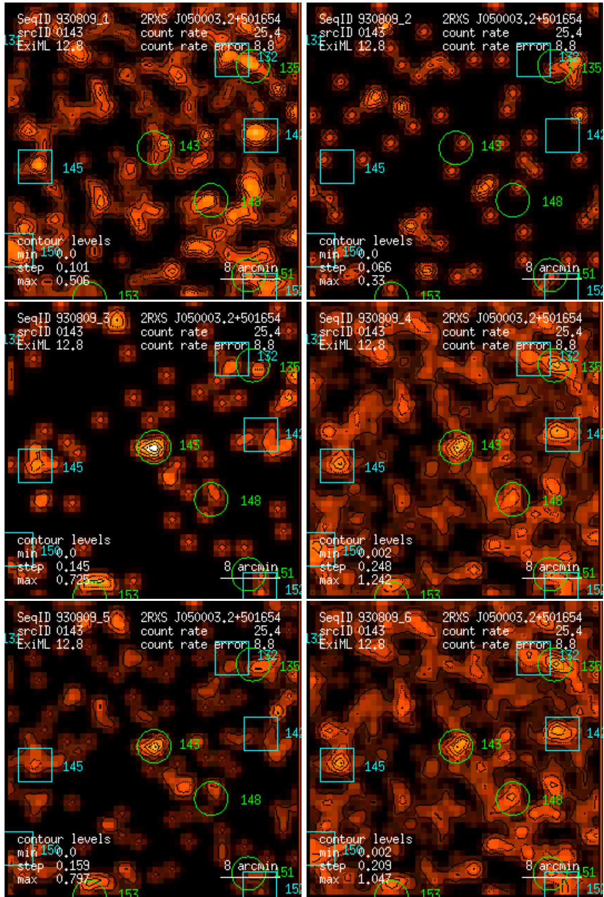
Figure 143: RASS 930809: detection 0143: band rate images, Gaussian filter: (1) PSPC channels 11 – 41, (2) 52 – 90, (3) 91 – 201, (4) 11 – 235, (5) 52 – 201, (6) 11 – 201. Broad band rates in counts/ks. Band rate contour levels in counts/ks/arcmin 2 .
