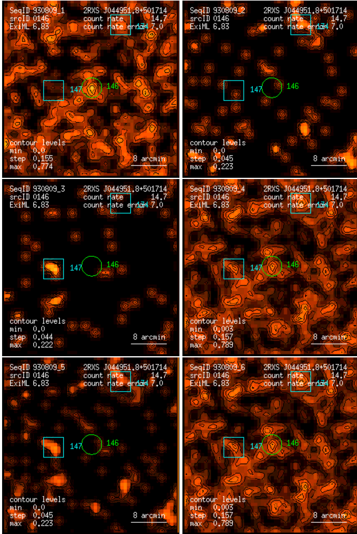
Figure 146: RASS 930809: detection 0146: band rate images, Gaussian filter: (1) PSPC channels 11 – 41, (2) 52 – 90, (3) 91 – 201, (4) 11 – 235, (5) 52 – 201, (6) 11 – 201. Broad band rates in counts/ks. Band rate contour levels in counts/ks/arcmin 2 .
