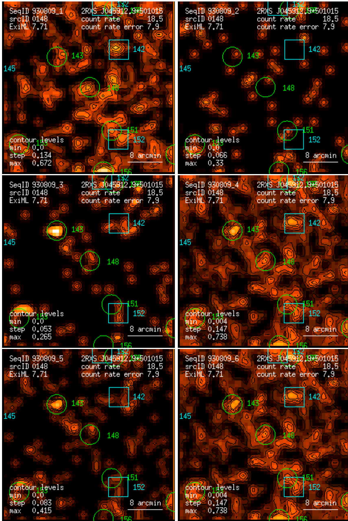
Figure 148: RASS 930809: detection 0148: band rate images, Gaussian filter: (1) PSPC channels 11 – 41, (2) 52 – 90, (3) 91 – 201, (4) 11 – 235, (5) 52 – 201, (6) 11 – 201. Broad band rates in counts/ks. Band rate contour levels in counts/ks/arcmin 2 .
