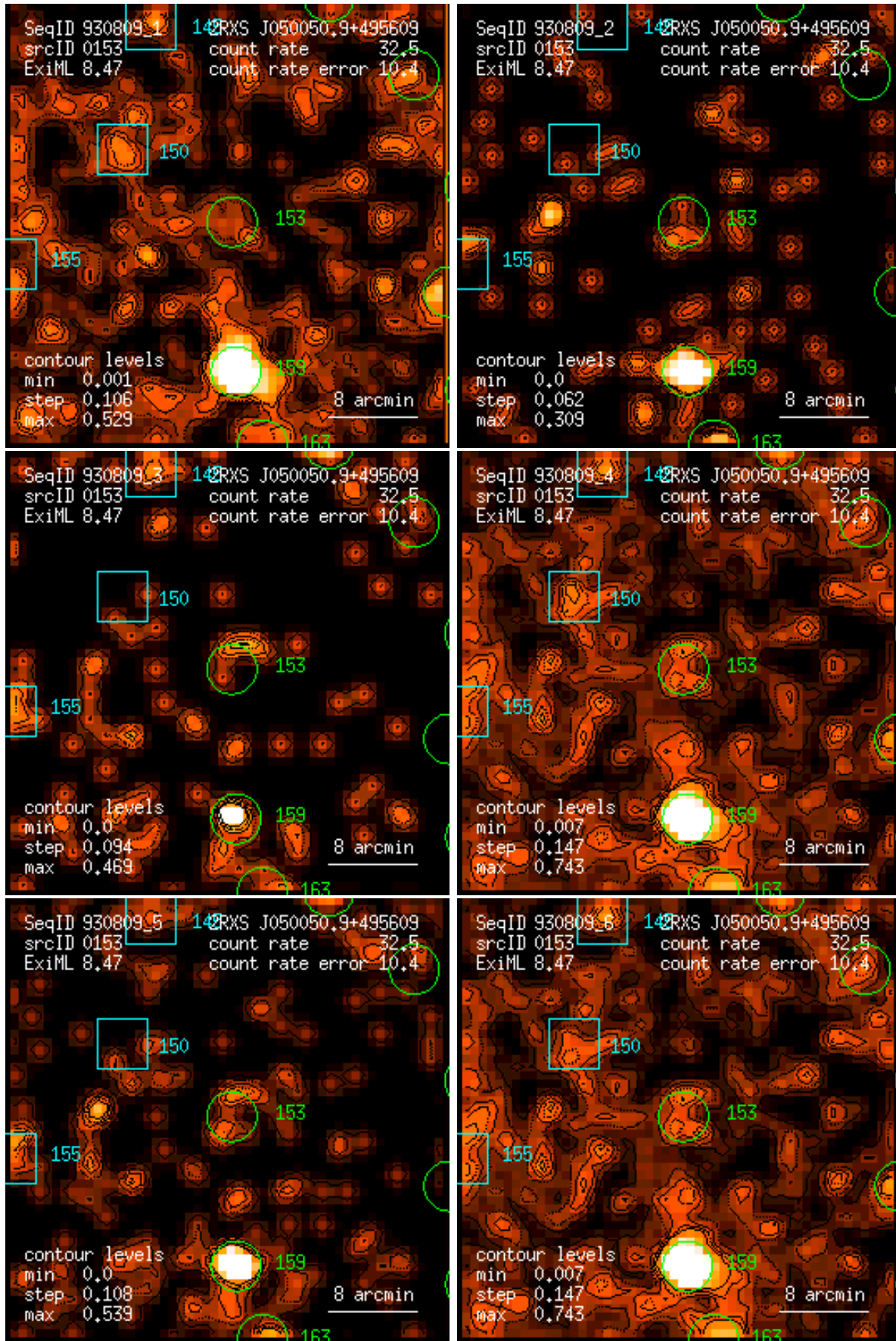
Figure 153: RASS 930809: detection 0153: band rate images, Gaussian filter: (1) PSPC channels 11 – 41, (2) 52 – 90, (3) 91 – 201, (4) 11 – 235, (5) 52 – 201, (6) 11 – 201. Broad band rates in counts/ks. Band rate contour levels in counts/ks/arcmin 2 .
