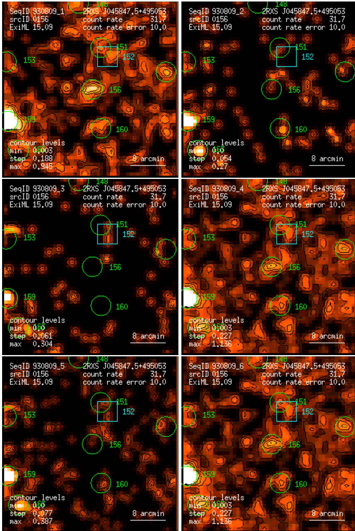
Figure 156: RASS 930809: detection 0156: band rate images, Gaussian filter: (1) PSPC channels 11 – 41, (2) 52 – 90, (3) 91 – 201, (4) 11 – 235, (5) 52 – 201, (6) 11 – 201. Broad band rates in counts/ks. Band rate contour levels in counts/ks/arcmin 2 .
