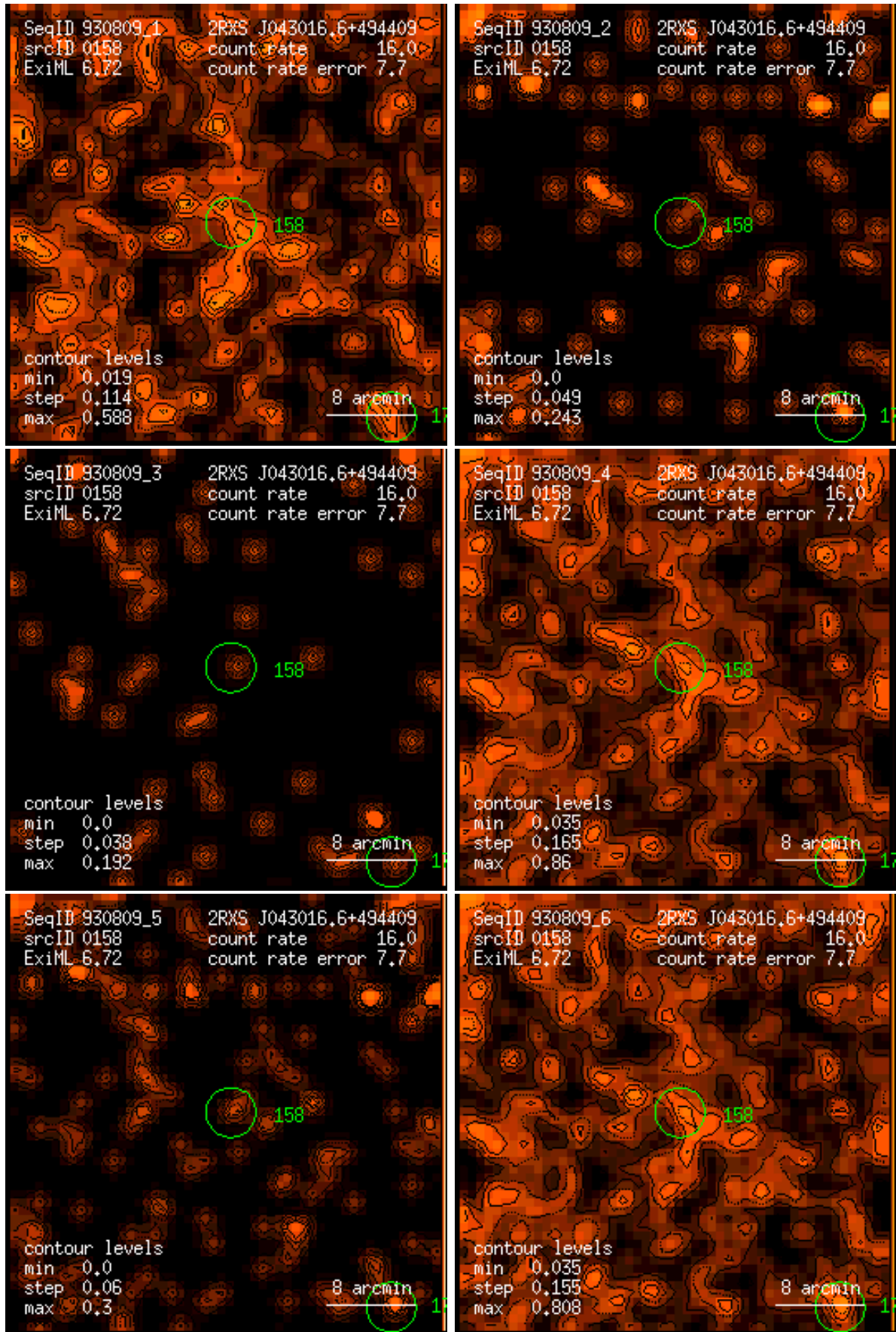
Figure 158: RASS 930809: detection 0158: band rate images, Gaussian filter: (1) PSPC channels 11 – 41, (2) 52 – 90, (3) 91 – 201, (4) 11 – 235, (5) 52 – 201, (6) 11 – 201. Broad band rates in counts/ks. Band rate contour levels in counts/ks/arcmin 2 .
