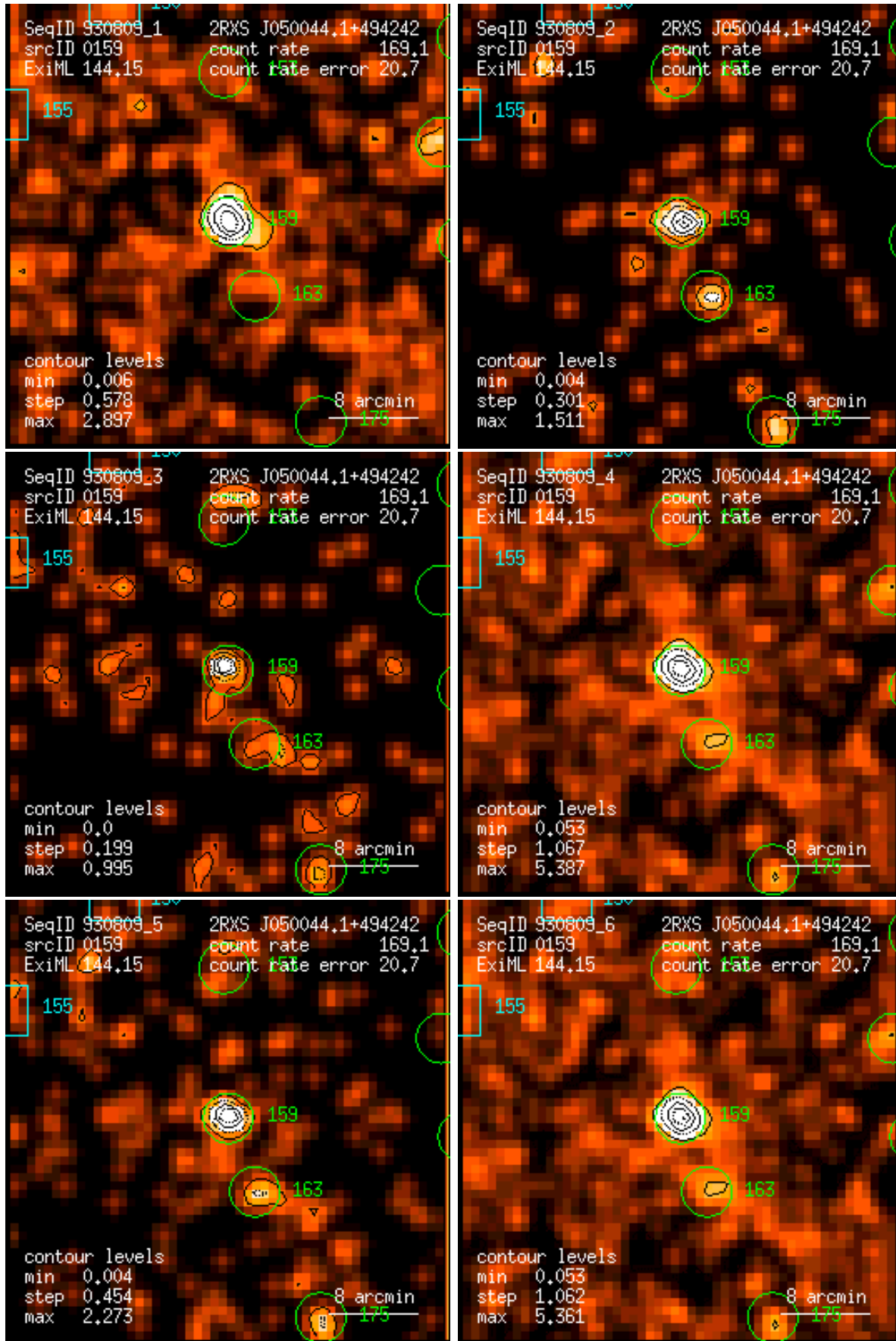
Figure 159: RASS 930809: detection 0159: band rate images, Gaussian filter: (1) PSPC channels 11 – 41, (2) 52 – 90, (3) 91 – 201, (4) 11 – 235, (5) 52 – 201, (6) 11 – 201. Broad band rates in counts/ks. Band rate contour levels in counts/ks/arcmin 2 .
